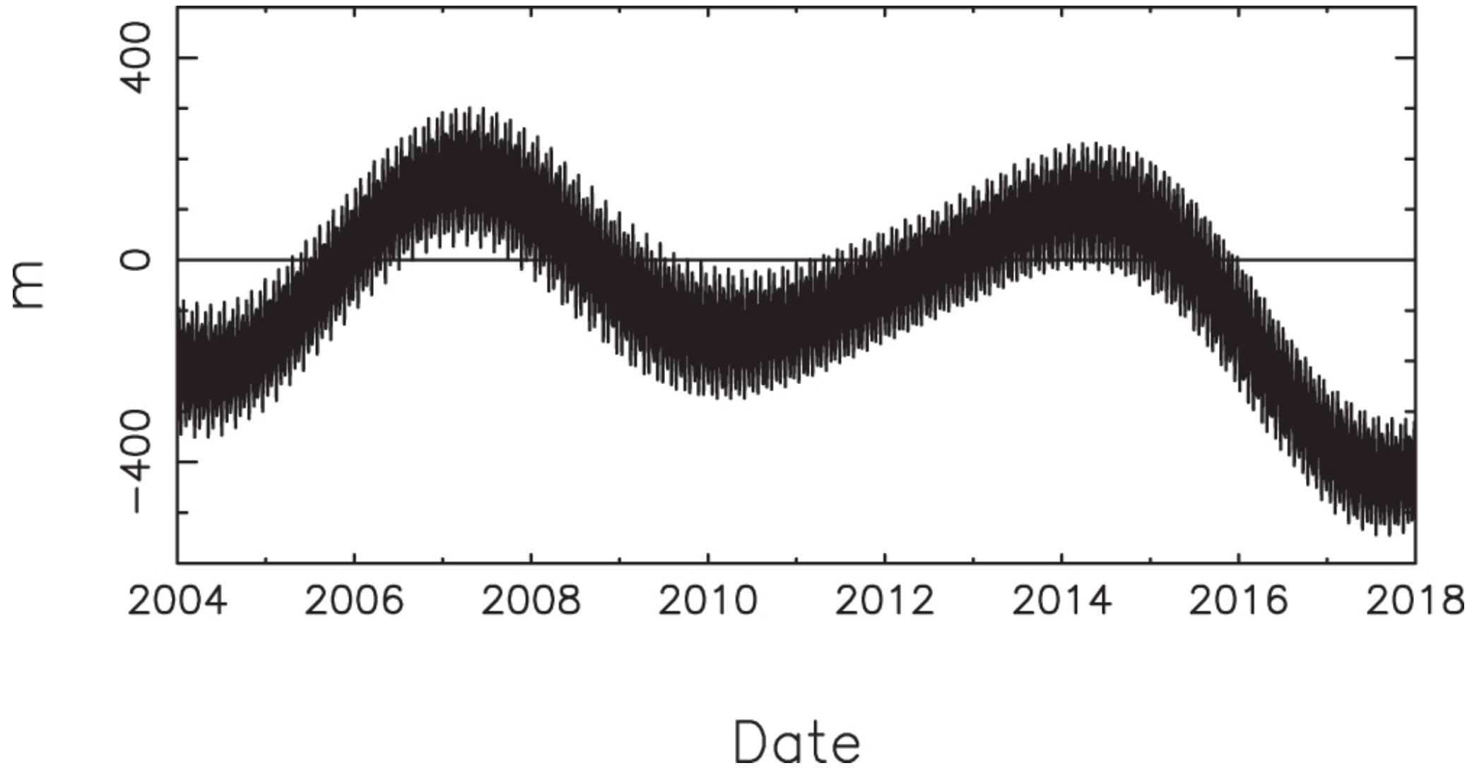
Figure 2. from Robert. A. Jacobson 2022 Astron. J. 164 doi:10.3847/1538-3881/ac90c9 https://dx.doi.org/10.3847/1538-3881/ac90c9 © 2022. The Author(s). Published by the American Astronomical Society.
