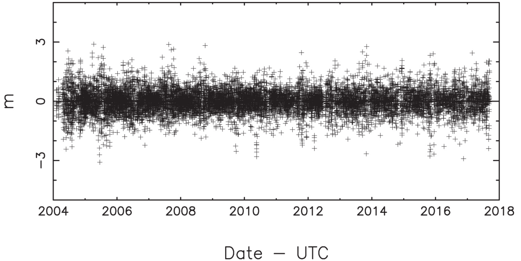
Figure 19. from Robert. A. Jacobson 2022 Astron. J. 164 doi:10.3847/1538-3881/ac90c9 https://dx.doi.org/10.3847/1538-3881/ac90c9 © 2022. The Author(s). Published by the American Astronomical Society.
