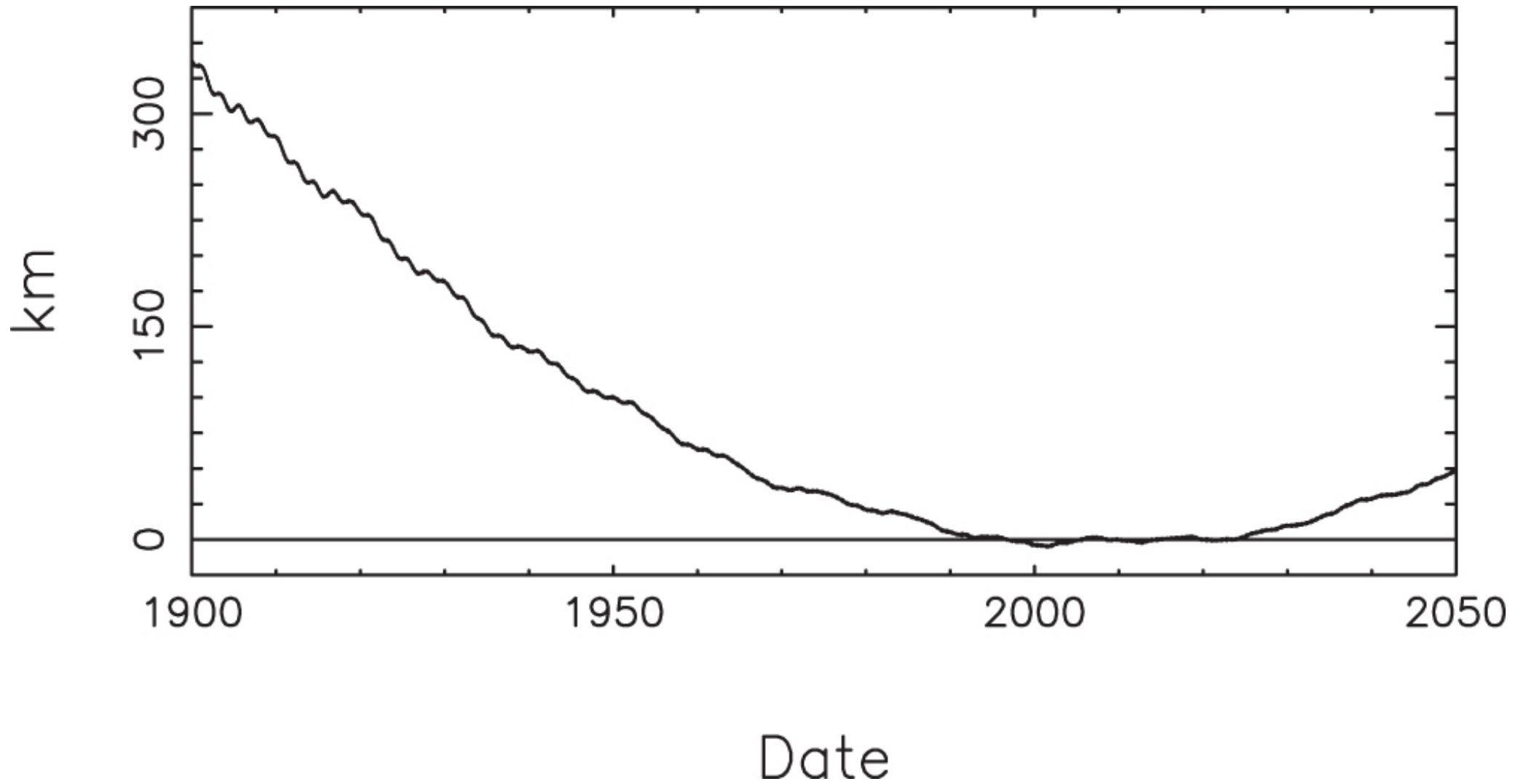
Figure 10. from Robert. A. Jacobson 2022 Astron. J. 164 doi:10.3847/1538-3881/ac90c9 https://dx.doi.org/10.3847/1538-3881/ac90c9 © 2022. The Author(s). Published by the American Astronomical Society.
