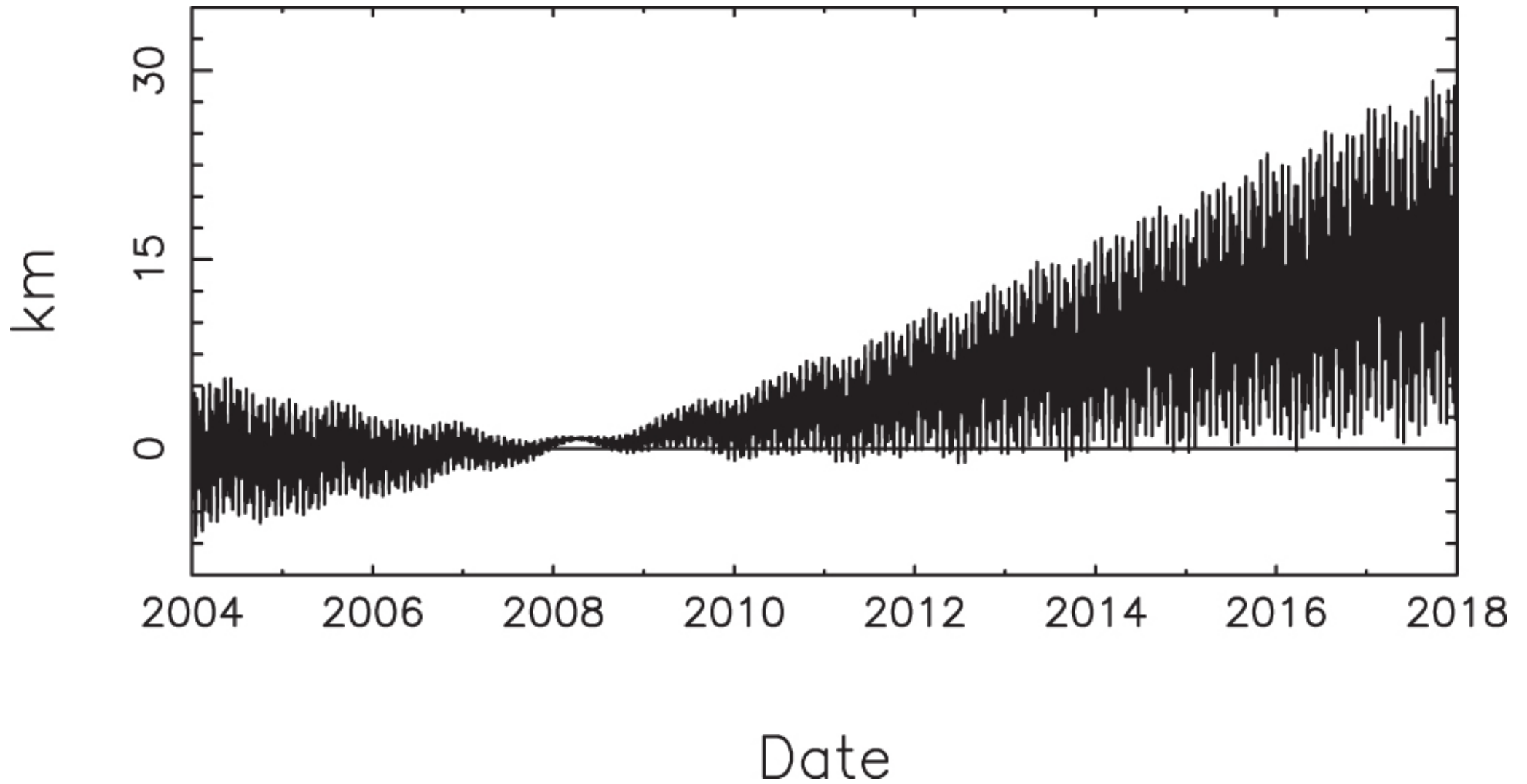
Figure 1. from Robert. A. Jacobson 2022 Astron. J. 164 doi:10.3847/1538-3881/ac90c9 https://dx.doi.org/10.3847/1538-3881/ac90c9 © 2022. The Author(s). Published by the American Astronomical Society.
