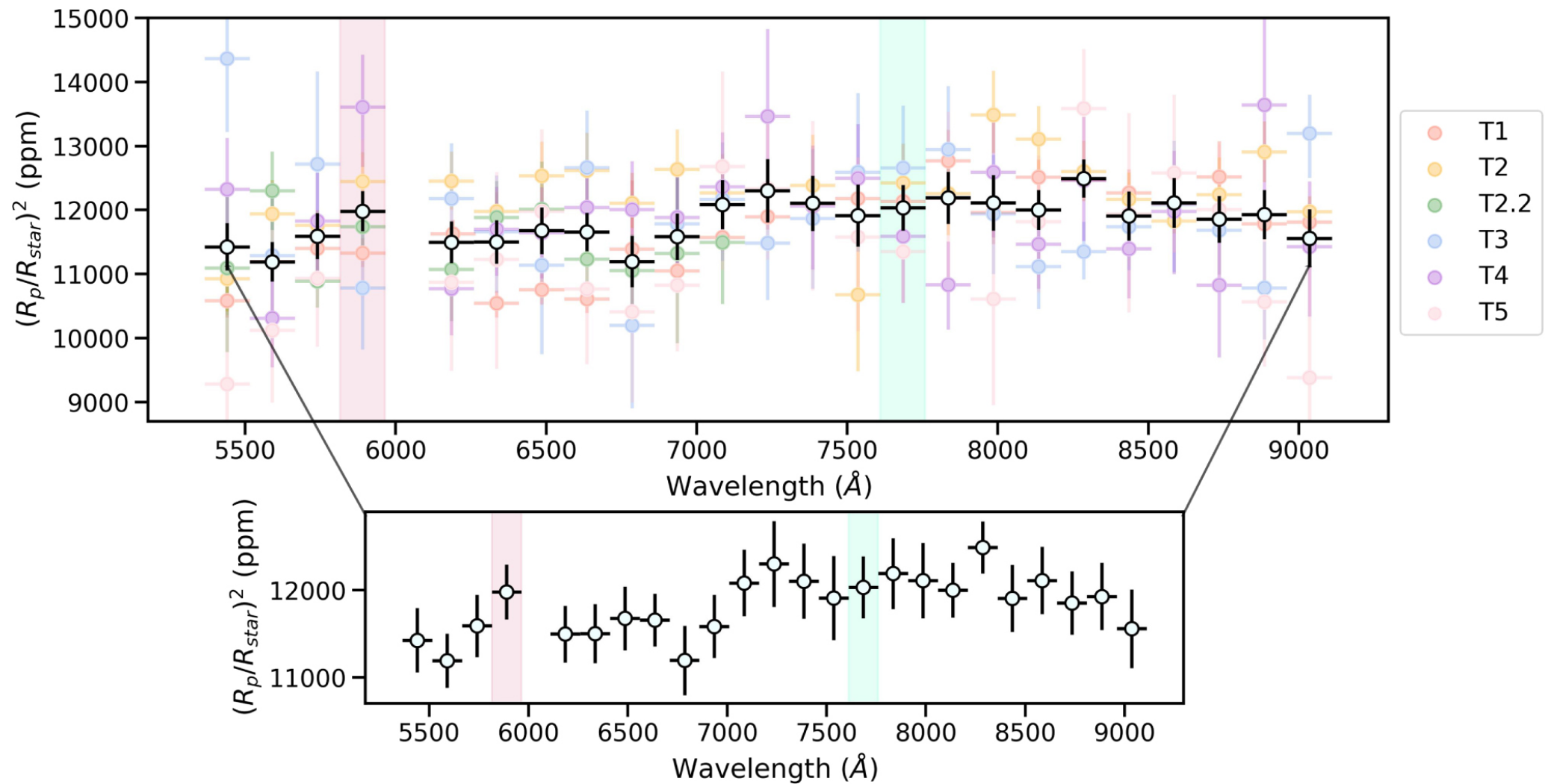
Figure 4. from Natalie H. Allen et al 2022 Astron. J. 164 doi:10.3847/1538-3881/ac8b74 https://dx.doi.org/10.3847/1538-3881/ac8b74 © 2022. The Author(s). Published by the American Astronomical Society.
