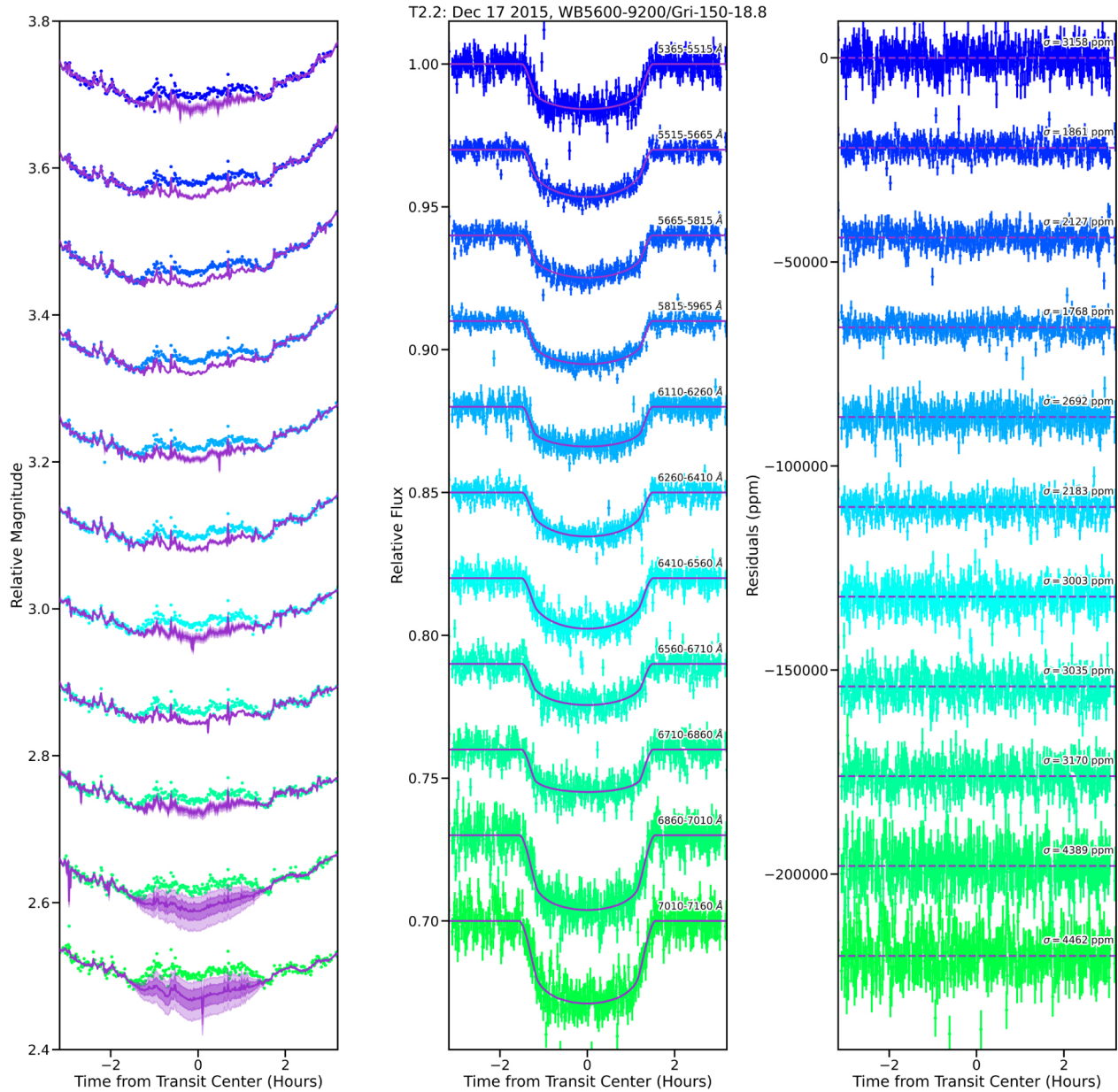
Figure 10. from Natalie H. Allen et al 2022 Astron. J. 164 doi:10.3847/1538-3881/ac8b74 https://dx.doi.org/10.3847/1538-3881/ac8b74 © 2022. The Author(s). Published by the American Astronomical Society.
