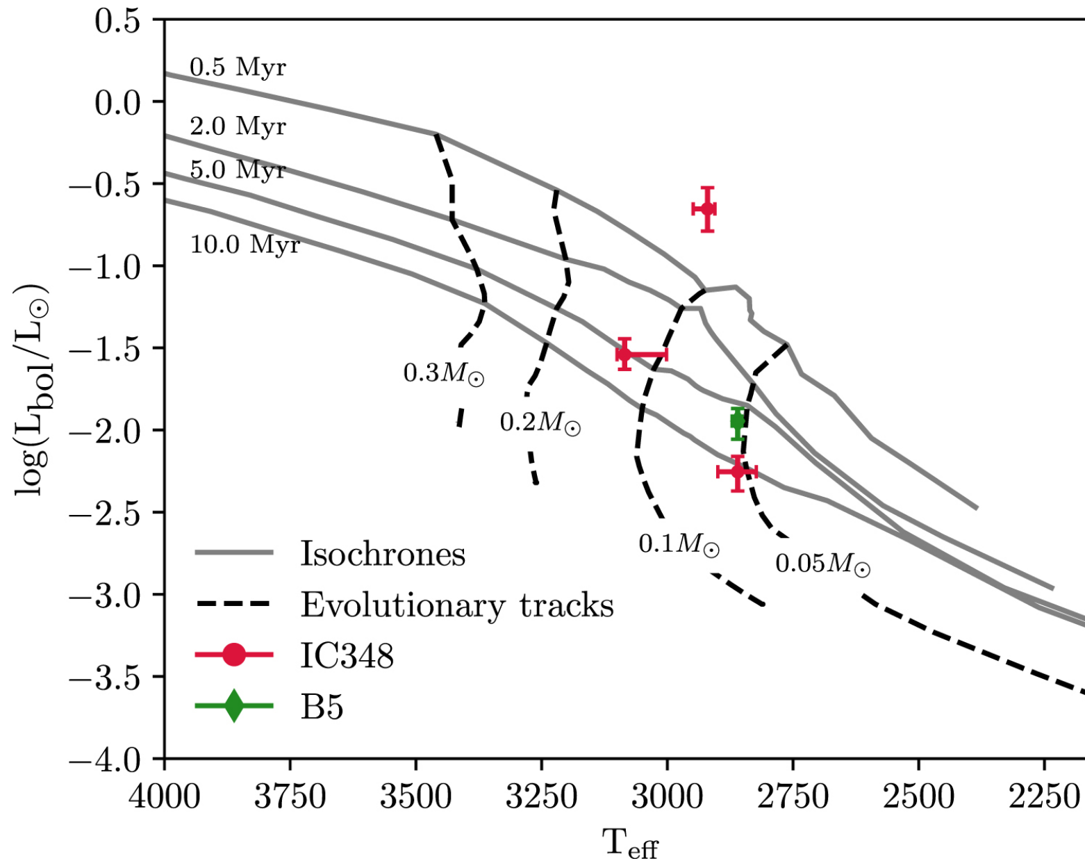
Figure 8. from Bhavana Lalchand et al 2022 Astron. J. 164 doi:10.3847/1538-3881/ac8547 https://dx.doi.org/10.3847/1538-3881/ac8547 © 2022. The Author(s). Published by the American Astronomical Society.
