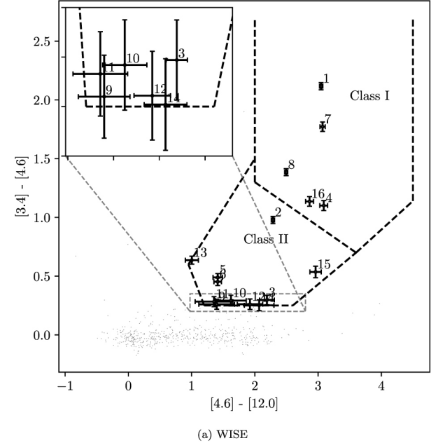
Figure 10. from Bhavana Lalchand et al 2022 Astron. J. 164 doi:10.3847/1538-3881/ac8547 https://dx.doi.org/10.3847/1538-3881/ac8547 © 2022. The Author(s). Published by the American Astronomical Society.
