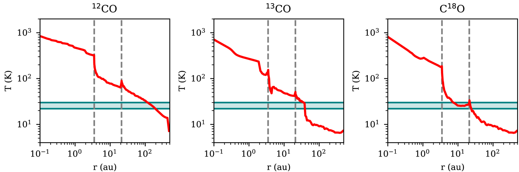
Figure 8. from Logan Francis et al 2022 Astron. J. 164 doi:10.3847/1538-3881/ac7ffb https://dx.doi.org/10.3847/1538-3881/ac7ffb © 2022. The Author(s). Published by the American Astronomical Society.
