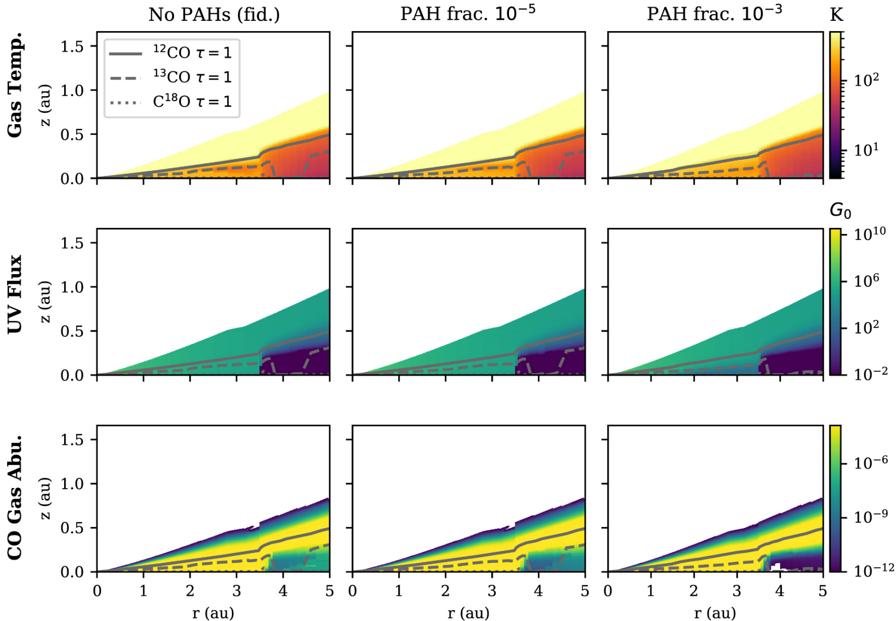
Figure 28. from Logan Francis et al 2022 Astron. J. 164 doi:10.3847/1538-3881/ac7ffb https://dx.doi.org/10.3847/1538-3881/ac7ffb © 2022. The Author(s). Published by the American Astronomical Society.
