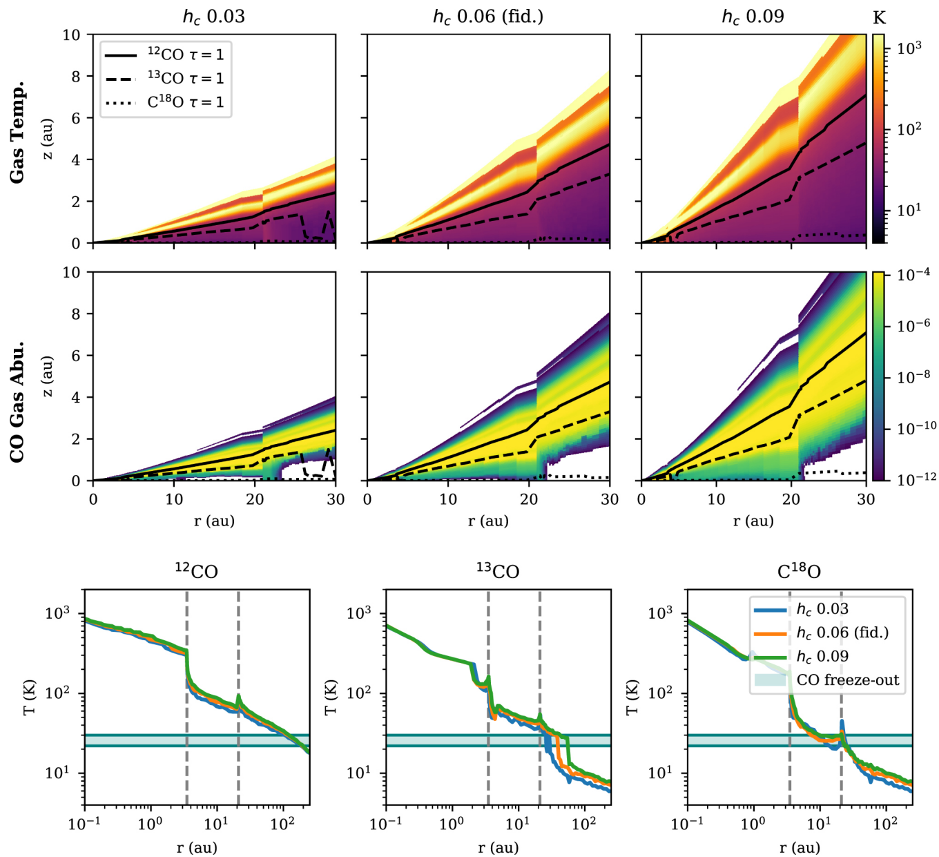
Figure 26. from Logan Francis et al 2022 Astron. J. 164 doi:10.3847/1538-3881/ac7ffb https://dx.doi.org/10.3847/1538-3881/ac7ffb © 2022. The Author(s). Published by the American Astronomical Society.
