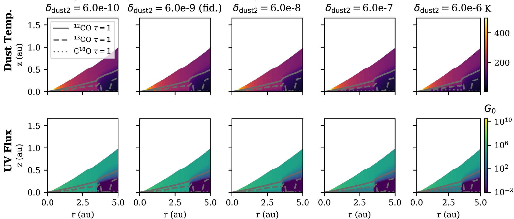
Figure 22. from Logan Francis et al 2022 Astron. J. 164 doi:10.3847/1538-3881/ac7ffb https://dx.doi.org/10.3847/1538-3881/ac7ffb © 2022. The Author(s). Published by the American Astronomical Society.
