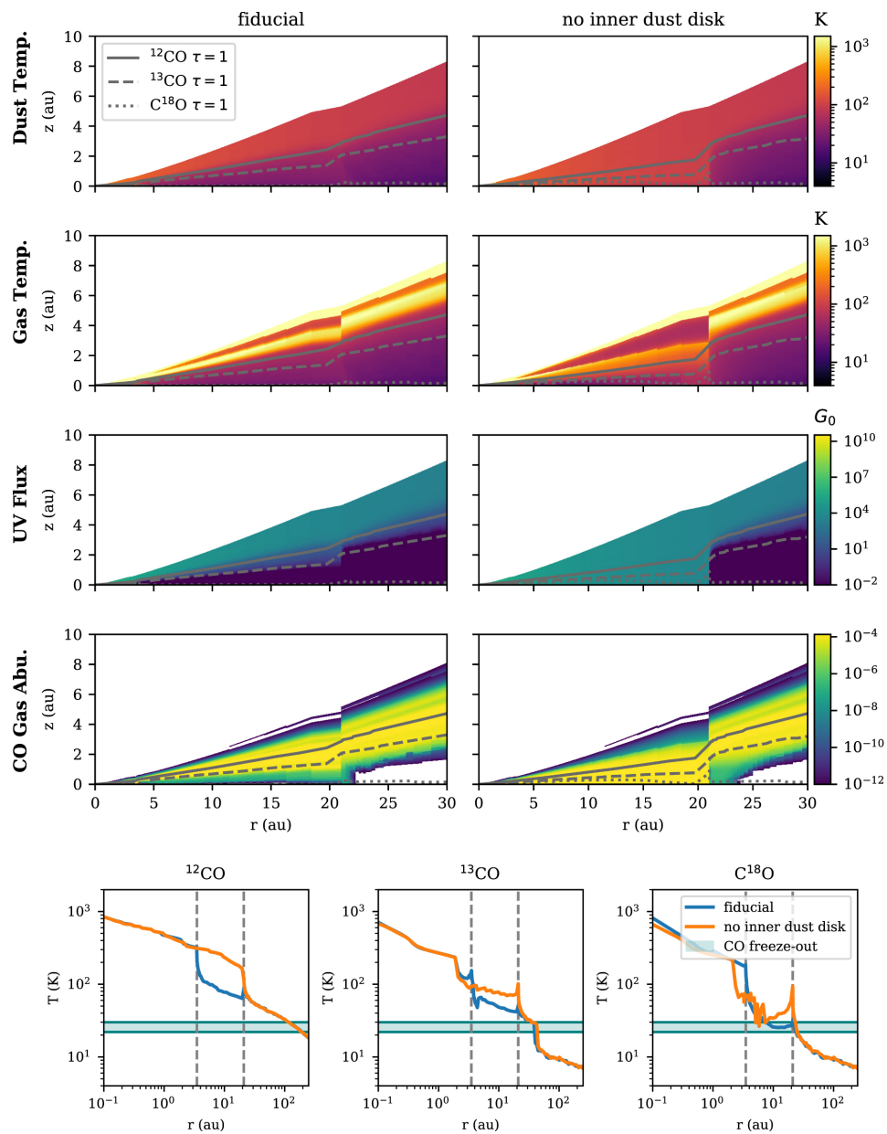
Figure 21. from Logan Francis et al 2022 Astron. J. 164 doi:10.3847/1538-3881/ac7ffb https://dx.doi.org/10.3847/1538-3881/ac7ffb © 2022. The Author(s). Published by the American Astronomical Society.
