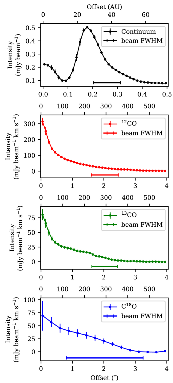
Figure 2. from Logan Francis et al 2022 Astron. J. 164 doi:10.3847/1538-3881/ac7ffb https://dx.doi.org/10.3847/1538-3881/ac7ffb © 2022. The Author(s). Published by the American Astronomical Society.
