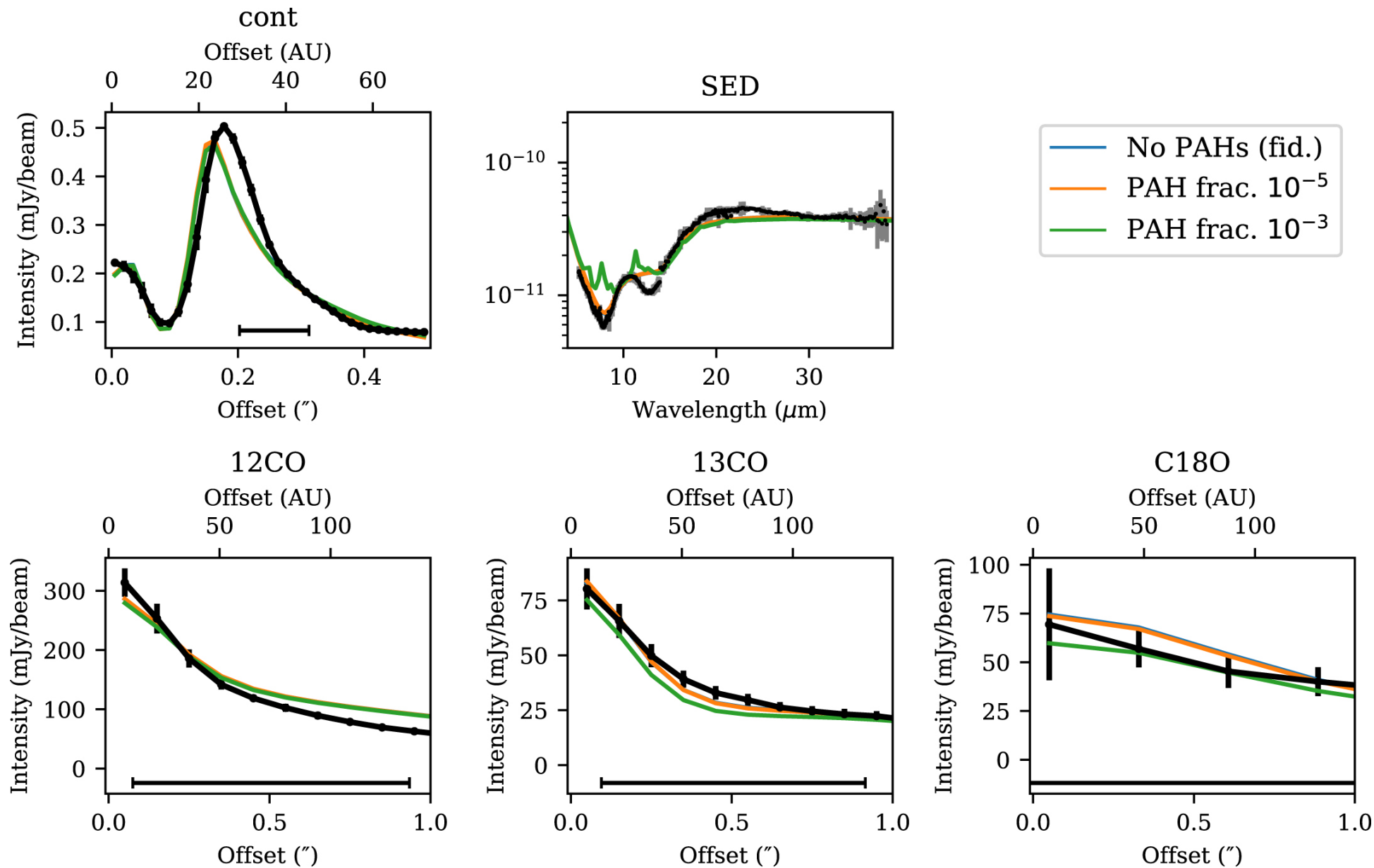
Figure 17. from Logan Francis et al 2022 Astron. J. 164 doi:10.3847/1538-3881/ac7ffb https://dx.doi.org/10.3847/1538-3881/ac7ffb © 2022. The Author(s). Published by the American Astronomical Society.
