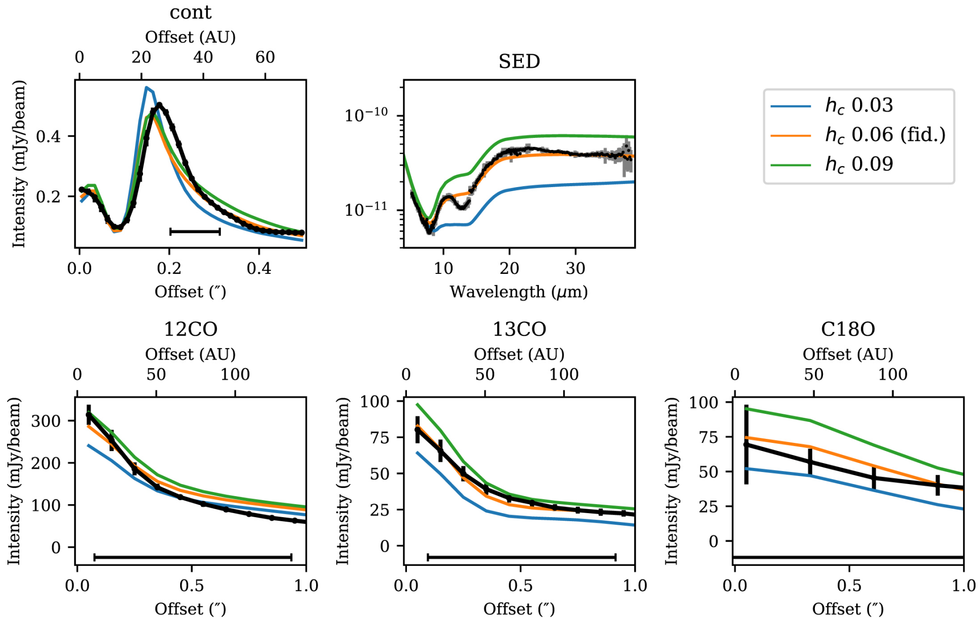
Figure 15. from Logan Francis et al 2022 Astron. J. 164 doi:10.3847/1538-3881/ac7ffb https://dx.doi.org/10.3847/1538-3881/ac7ffb © 2022. The Author(s). Published by the American Astronomical Society.
