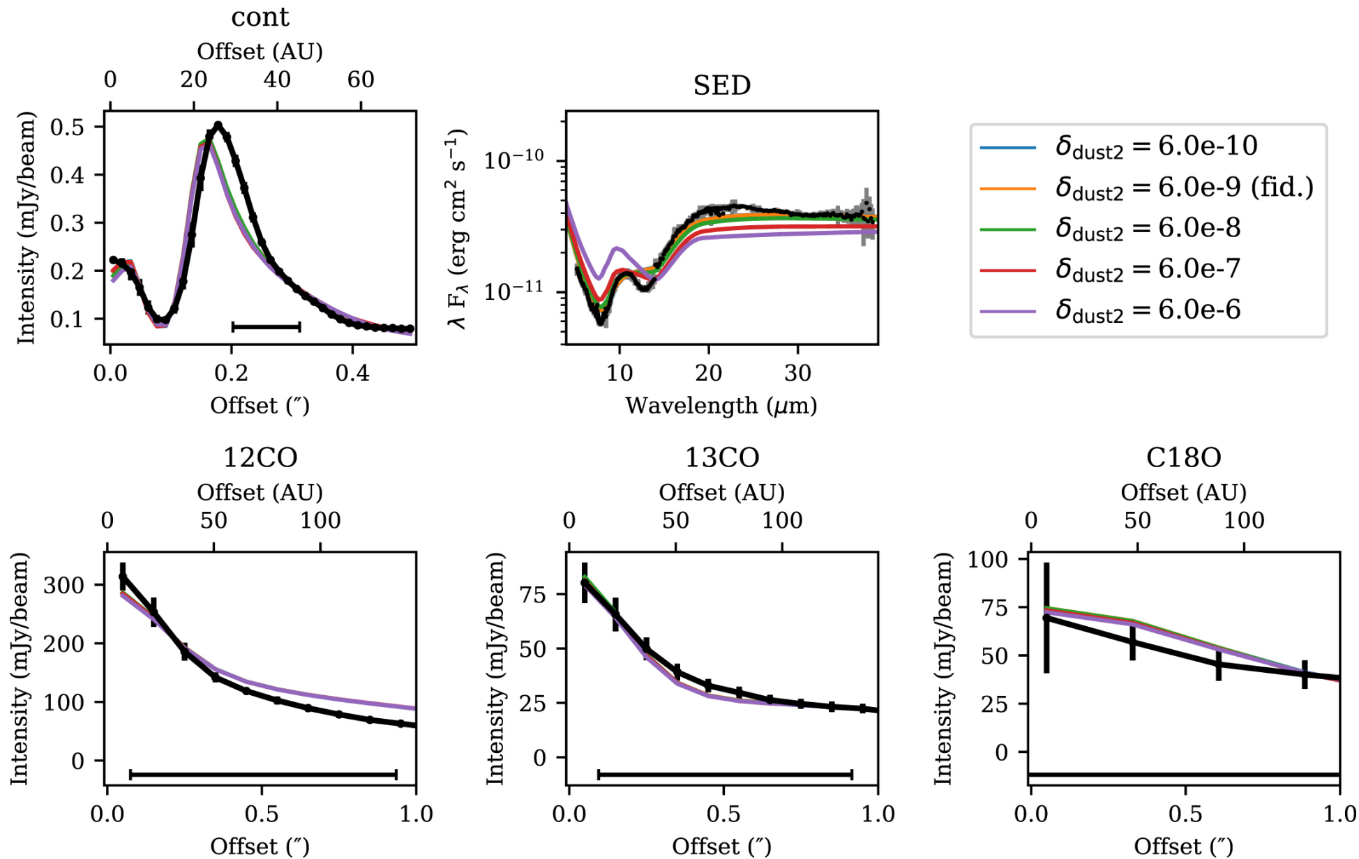
Figure 10. from Logan Francis et al 2022 Astron. J. 164 doi:10.3847/1538-3881/ac7ffb https://dx.doi.org/10.3847/1538-3881/ac7ffb © 2022. The Author(s). Published by the American Astronomical Society.
