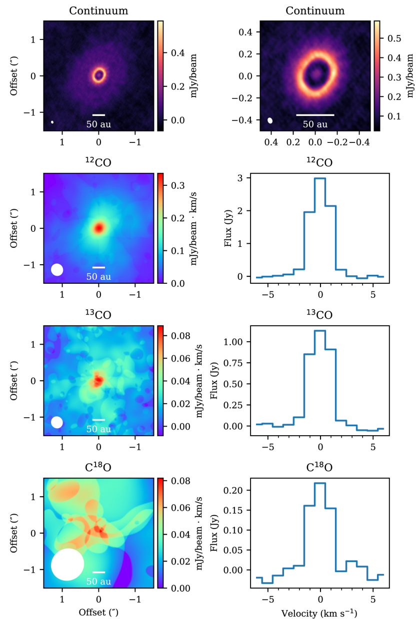
Figure 1. from Logan Francis et al 2022 Astron. J. 164 doi:10.3847/1538-3881/ac7ffb https://dx.doi.org/10.3847/1538-3881/ac7ffb © 2022. The Author(s). Published by the American Astronomical Society.
