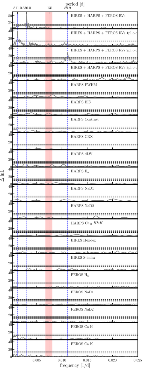
Figure 2. from Trifon Trifonov et al 2022 Astron. J. 164 doi:10.3847/1538-3881/ac7ce0 https://dx.doi.org/10.3847/1538-3881/ac7ce0 © 2022. The Author(s). Published by the American Astronomical Society.
