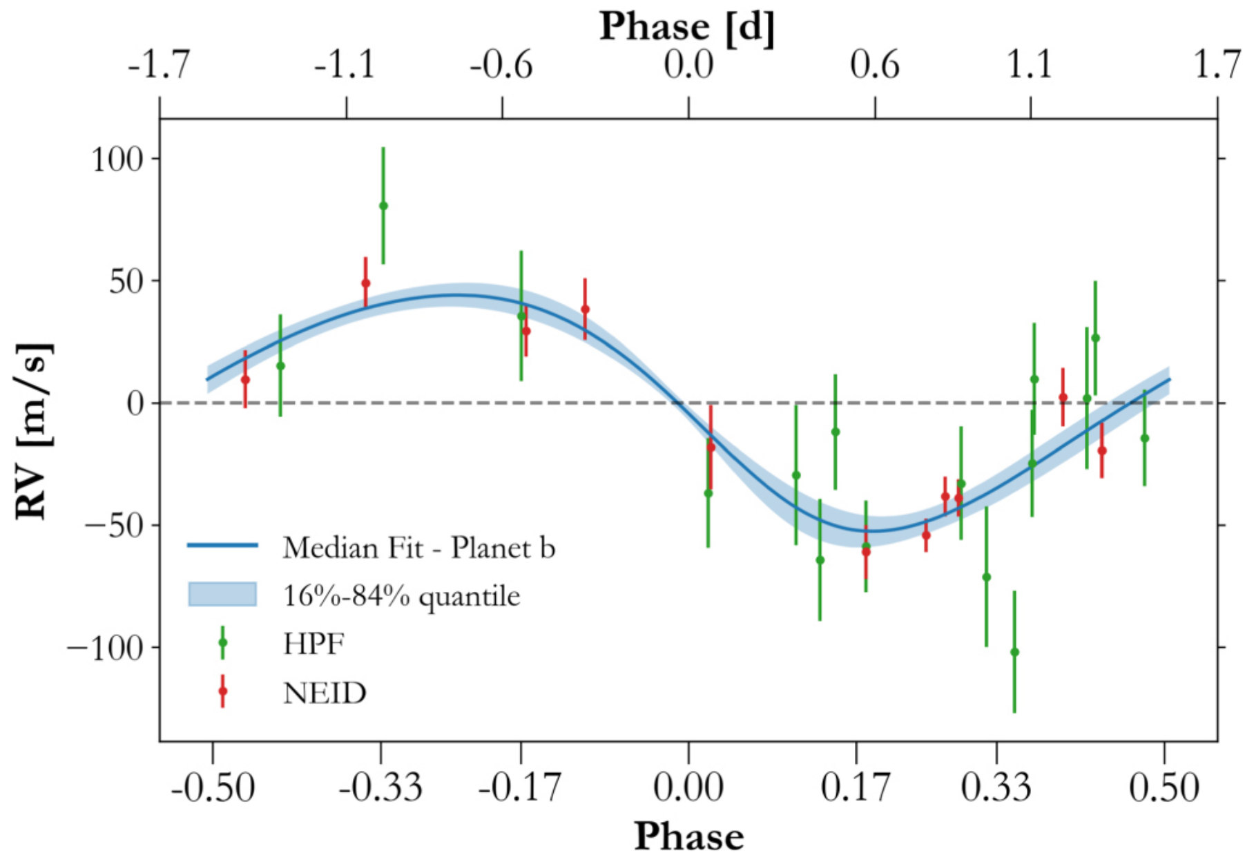
Figure 7. from Shubham Kanodia et al 2022 Astron. J. 164 doi:10.3847/1538-3881/ac7c20 https://dx.doi.org/10.3847/1538-3881/ac7c20 © 2022. The Author(s). Published by the American Astronomical Society.
