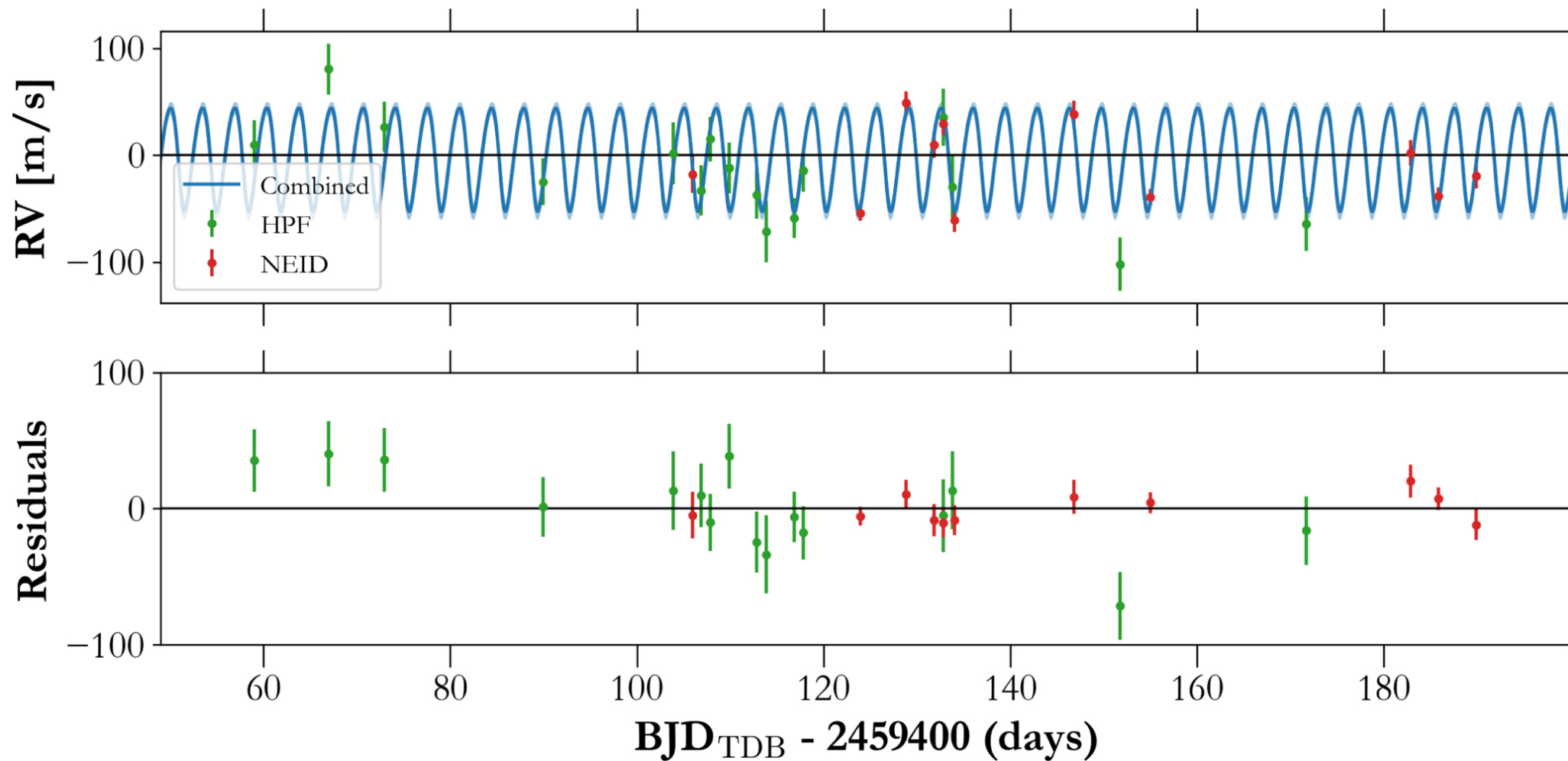
Figure 3. from Shubham Kanodia et al 2022 Astron. J. 164 doi:10.3847/1538-3881/ac7c20 https://dx.doi.org/10.3847/1538-3881/ac7c20 © 2022. The Author(s). Published by the American Astronomical Society.
