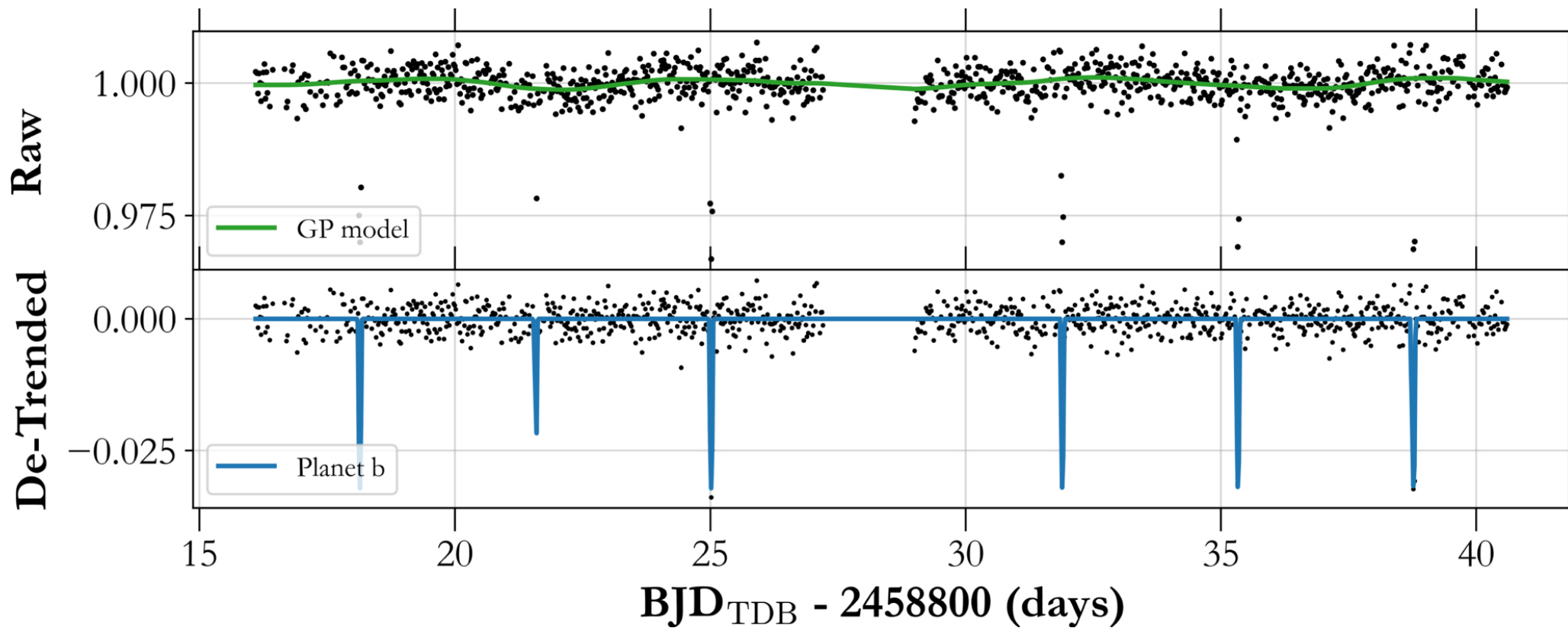
Figure 1. from Shubham Kanodia et al 2022 Astron. J. 164 doi:10.3847/1538-3881/ac7c20 https://dx.doi.org/10.3847/1538-3881/ac7c20 © 2022. The Author(s). Published by the American Astronomical Society.
