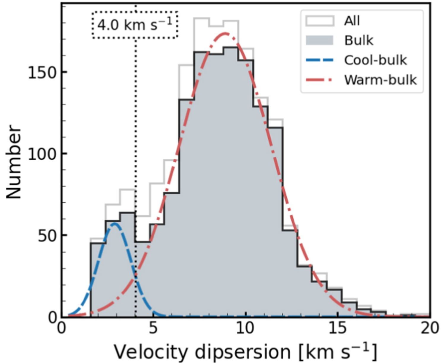
Figure 8. from Hye-Jin Park et al 2022 Astron. J. 164 doi:10.3847/1538-3881/ac7c1b https://dx.doi.org/10.3847/1538-3881/ac7c1b © 2022. The Author(s). Published by the American Astronomical Society.
