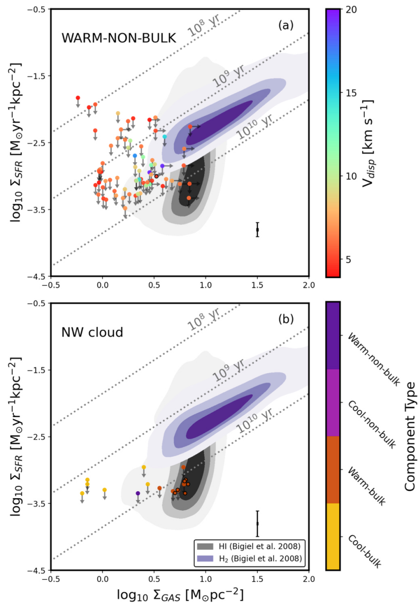
Figure 11. from Hye-Jin Park et al 2022 Astron. J. 164 doi:10.3847/1538-3881/ac7c1b https://dx.doi.org/10.3847/1538-3881/ac7c1b © 2022. The Author(s). Published by the American Astronomical Society.
