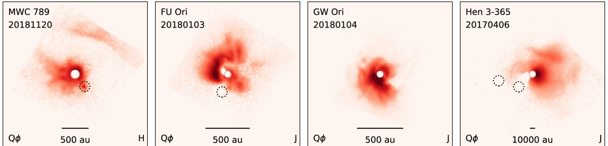
Figure 9. from Evan A. Rich et al 2022 Astron. J. 164 doi:10.3847/1538-3881/ac7be4 https://dx.doi.org/10.3847/1538-3881/ac7be4 © 2022. The Author(s). Published by the American Astronomical Society.
