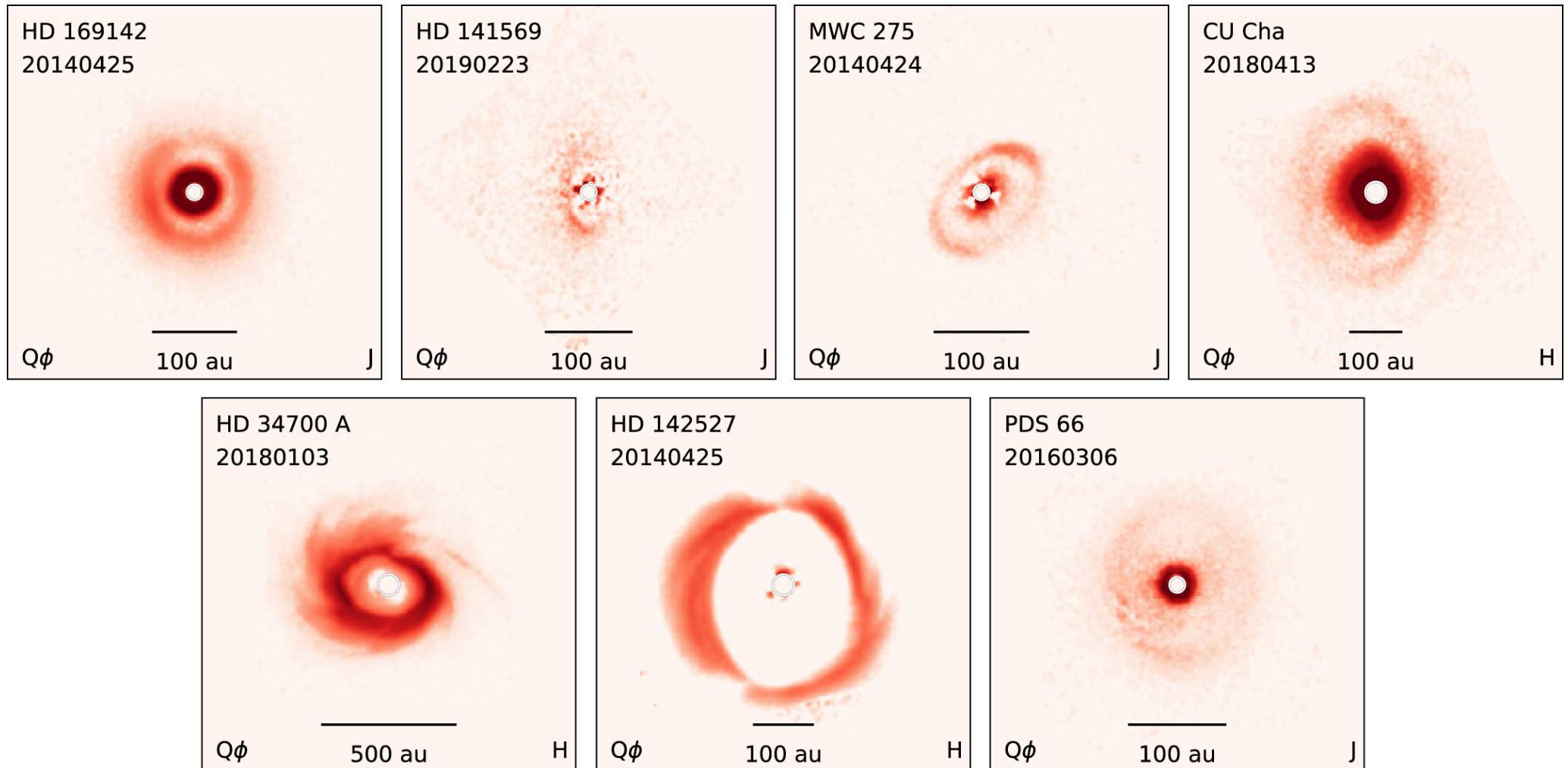
Figure 7. from Evan A. Rich et al 2022 Astron. J. 164 doi:10.3847/1538-3881/ac7be4 https://dx.doi.org/10.3847/1538-3881/ac7be4 © 2022. The Author(s). Published by the American Astronomical Society.
