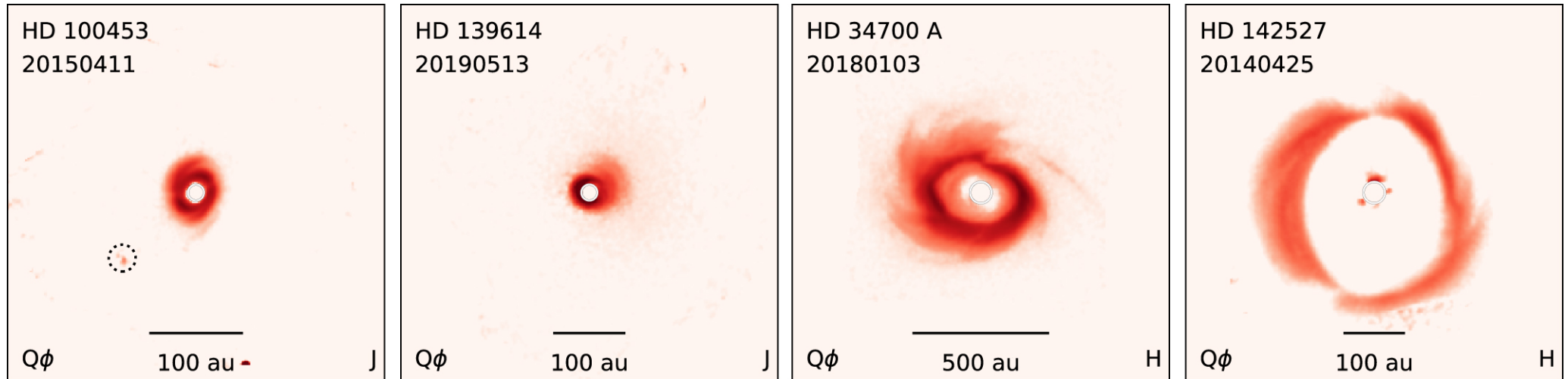
Figure 6. from Evan A. Rich et al 2022 Astron. J. 164 doi:10.3847/1538-3881/ac7be4 https://dx.doi.org/10.3847/1538-3881/ac7be4 © 2022. The Author(s). Published by the American Astronomical Society.
