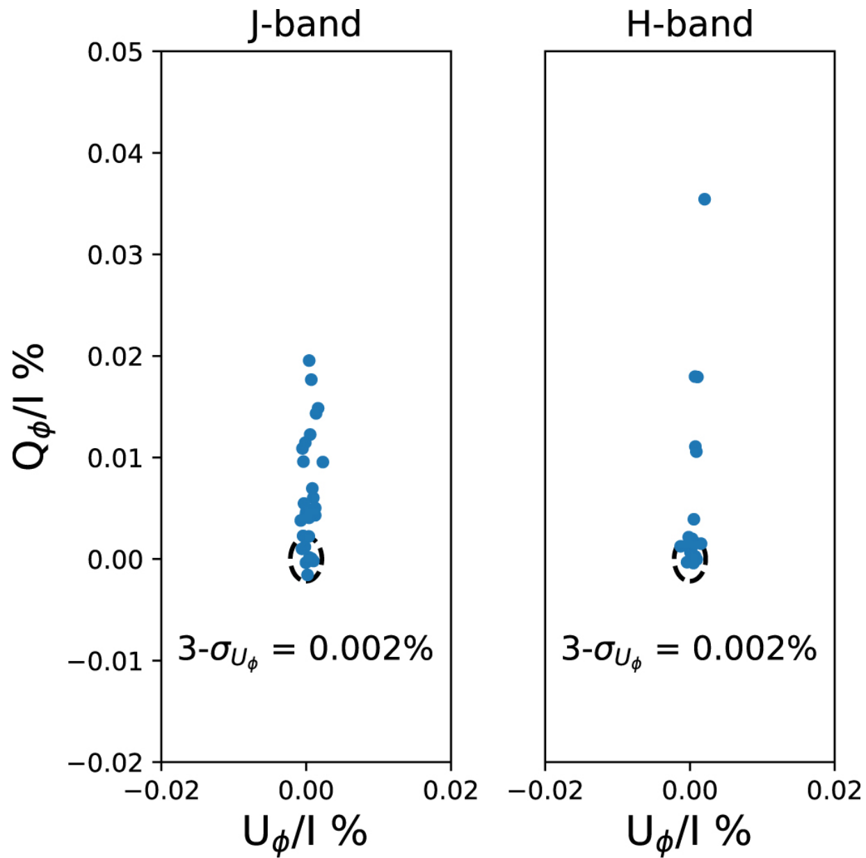
Figure 5. from Evan A. Rich et al 2022 Astron. J. 164 doi:10.3847/1538-3881/ac7be4 https://dx.doi.org/10.3847/1538-3881/ac7be4 © 2022. The Author(s). Published by the American Astronomical Society.
