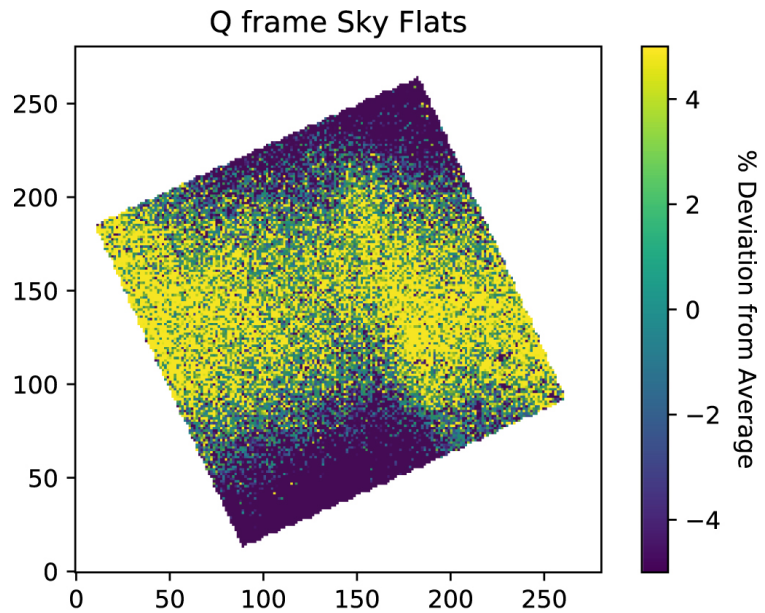
Figure 4. from Evan A. Rich et al 2022 Astron. J. 164 doi:10.3847/1538-3881/ac7be4 https://dx.doi.org/10.3847/1538-3881/ac7be4 © 2022. The Author(s). Published by the American Astronomical Society.
