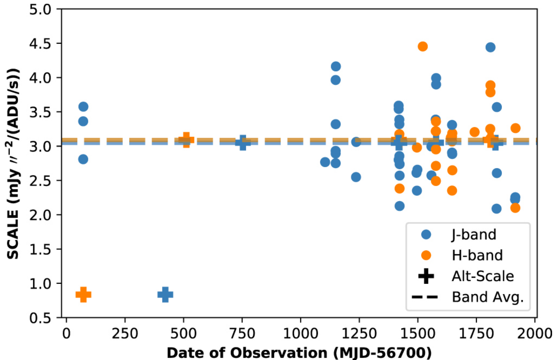
Figure 3. from Evan A. Rich et al 2022 Astron. J. 164 doi:10.3847/1538-3881/ac7be4 https://dx.doi.org/10.3847/1538-3881/ac7be4 © 2022. The Author(s). Published by the American Astronomical Society.
