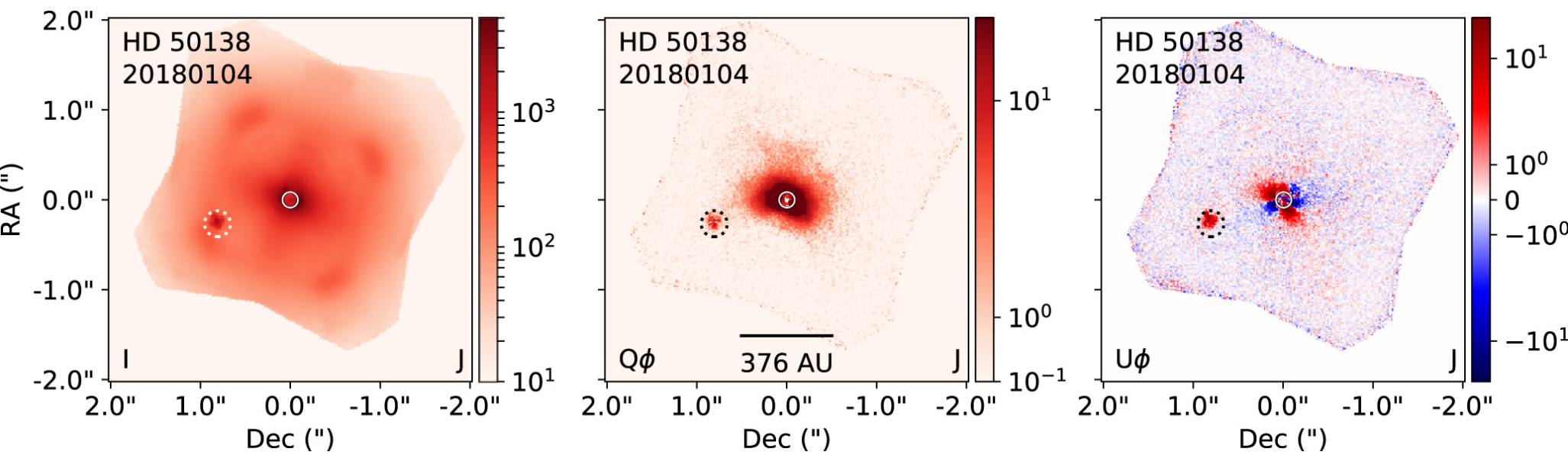
Figure 2. I, Q, and U images for all targets from Evan A. Rich et al 2022 Astron. J. 164 doi:10.3847/1538-3881/ac7be4 https://dx.doi.org/10.3847/1538-3881/ac7be4 © 2022. The Author(s). Published by the American Astronomical Society.
