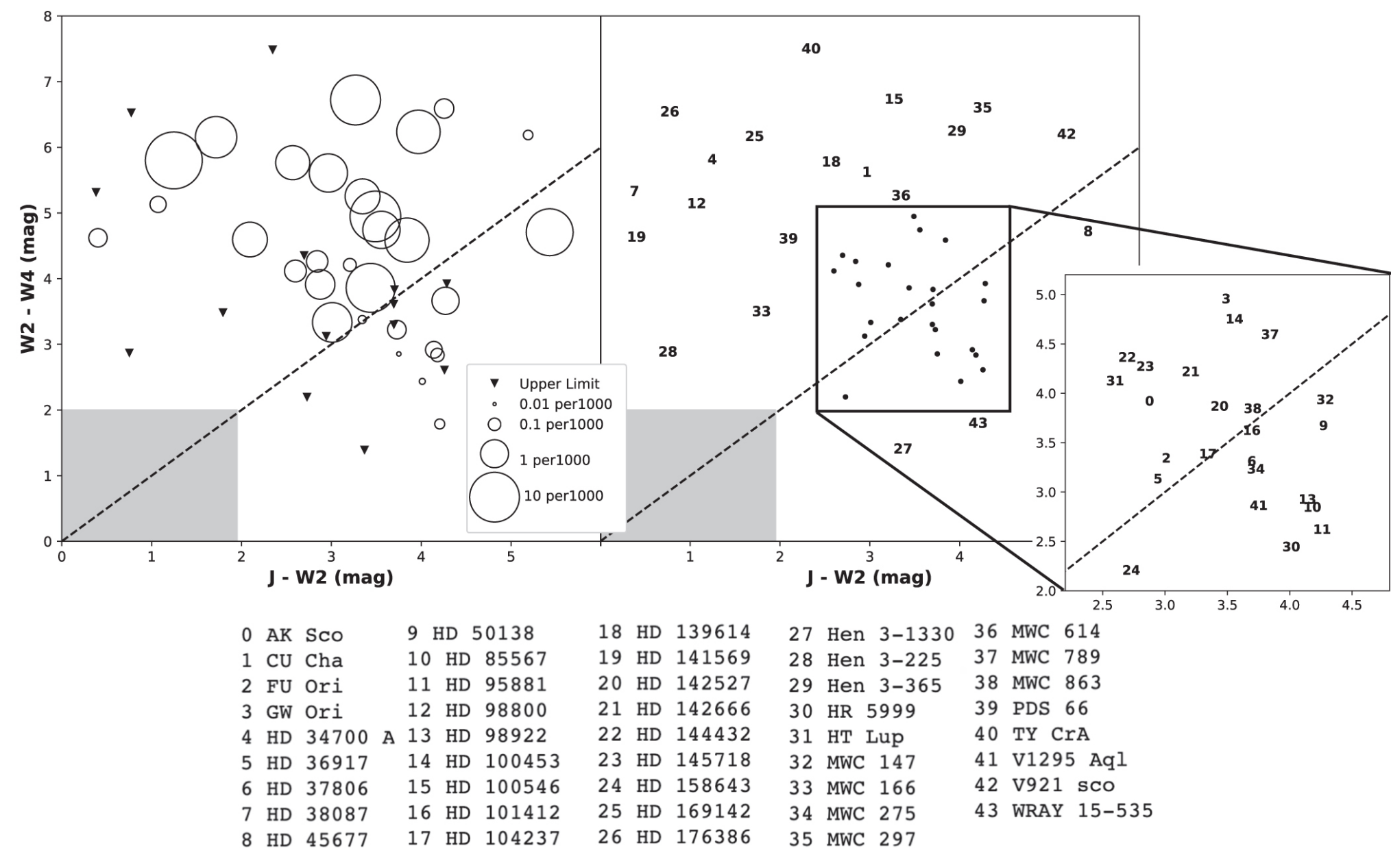
Figure 15. from Evan A. Rich et al 2022 Astron. J. 164 doi:10.3847/1538-3881/ac7be4 https://dx.doi.org/10.3847/1538-3881/ac7be4 © 2022. The Author(s). Published by the American Astronomical Society.
