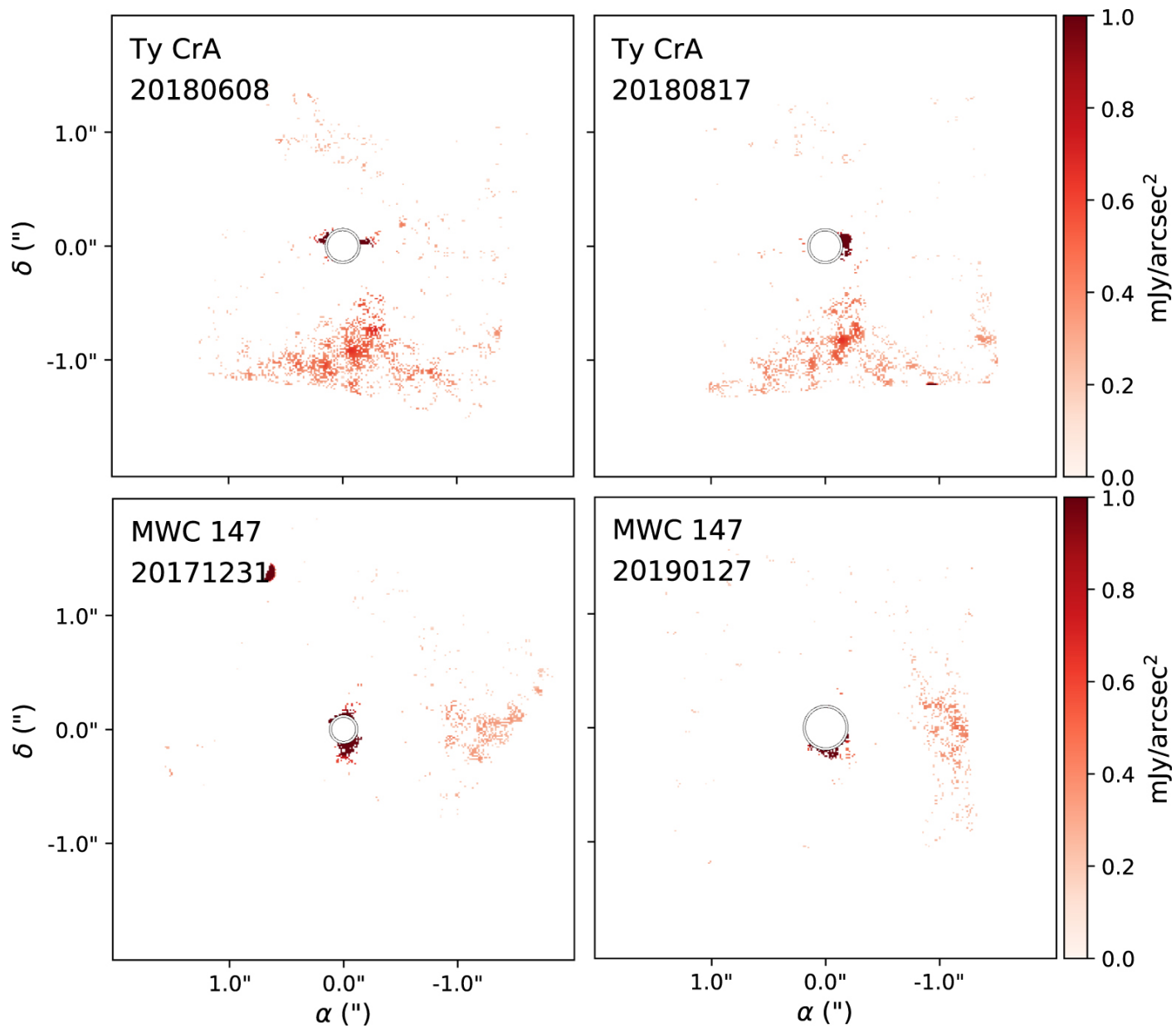
Figure 14. from Evan A. Rich et al 2022 Astron. J. 164 doi:10.3847/1538-3881/ac7be4 https://dx.doi.org/10.3847/1538-3881/ac7be4 © 2022. The Author(s). Published by the American Astronomical Society.
