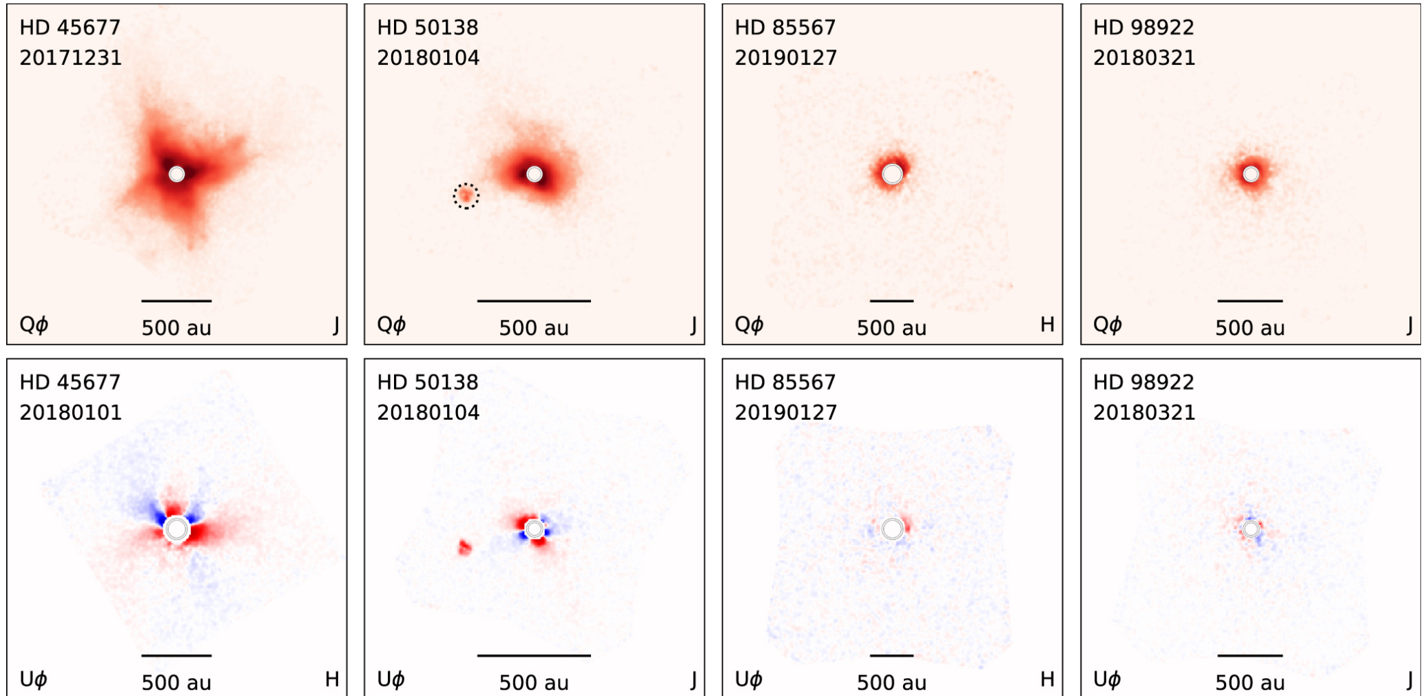
Figure 12. from Evan A. Rich et al 2022 Astron. J. 164 doi:10.3847/1538-3881/ac7be4 https://dx.doi.org/10.3847/1538-3881/ac7be4 © 2022. The Author(s). Published by the American Astronomical Society.
