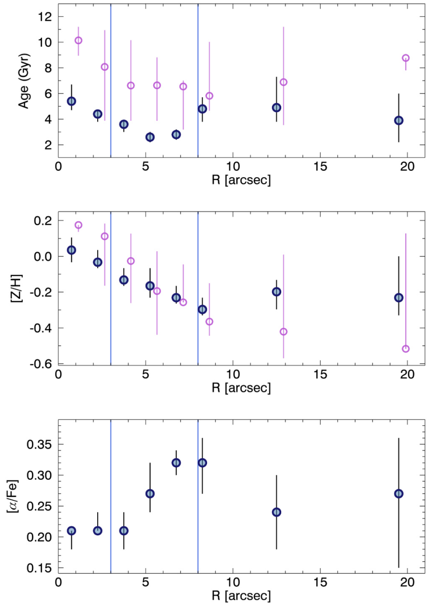
Figure 3. from Mina Pak et al 2023 Astron. J. 165 doi:10.3847/1538-3881/ac7b83 https://dx.doi.org/10.3847/1538-3881/ac7b83 © 2023. The Author(s). Published by the American Astronomical Society.
