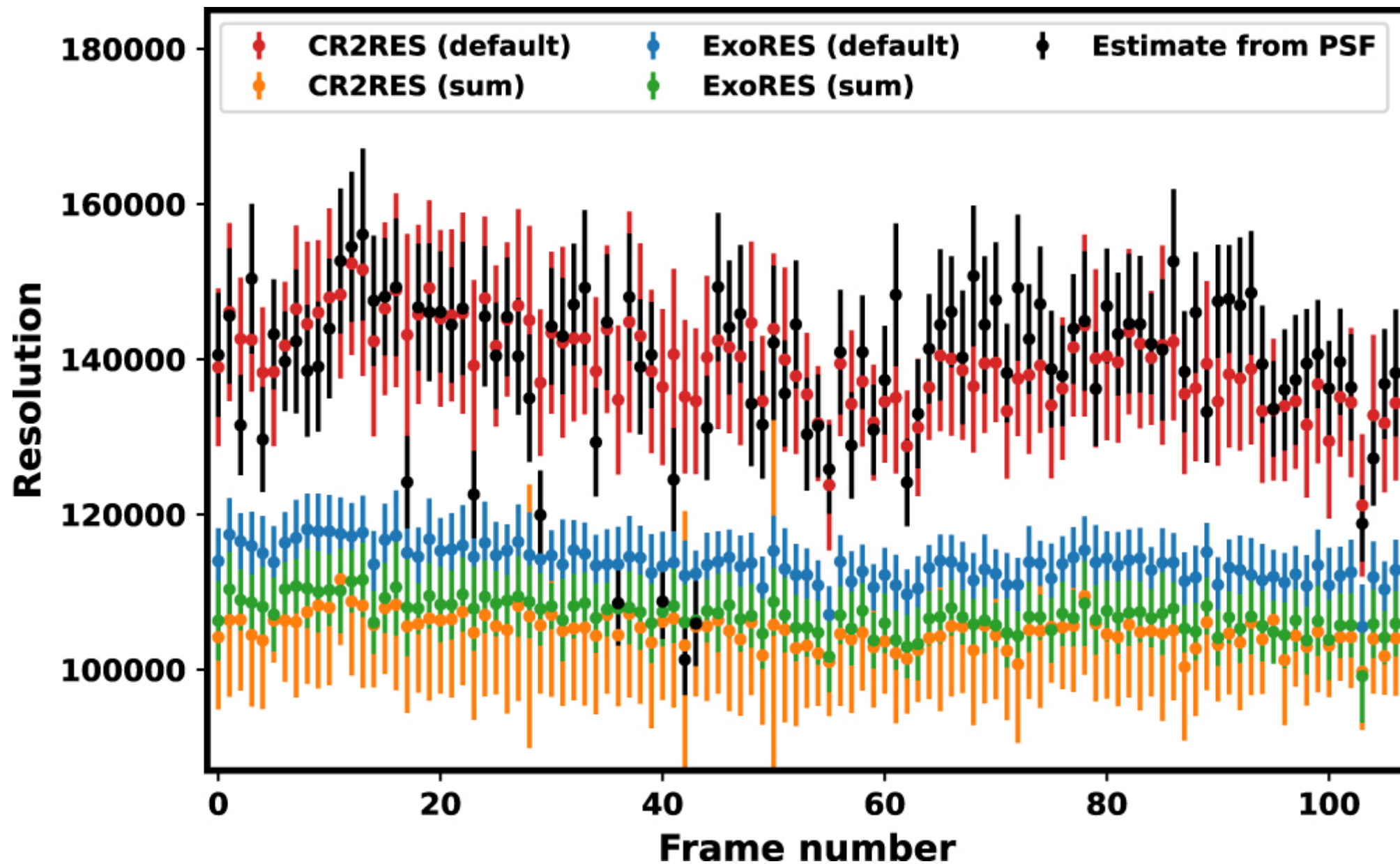
Figure 9. from Måns Holmberg and Nikku Madhusudhan 2022 Astron. J. 164 doi:10.3847/1538-3881/ac77eb https://dx.doi.org/10.3847/1538-3881/ac77eb © 2022. The Author(s). Published by the American Astronomical Society.
