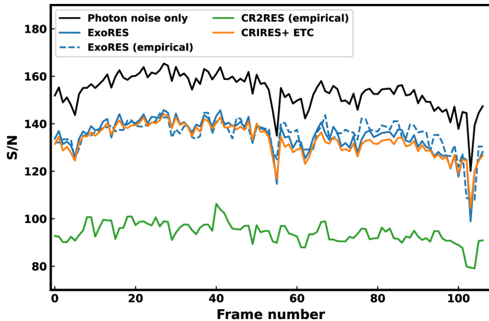
Figure 8. from Måns Holmberg and Nikku Madhusudhan 2022 Astron. J. 164 doi:10.3847/1538-3881/ac77eb https://dx.doi.org/10.3847/1538-3881/ac77eb © 2022. The Author(s). Published by the American Astronomical Society.
