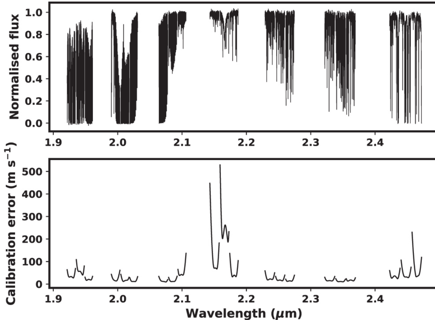
Figure 5. from Måns Holmberg and Nikku Madhusudhan 2022 Astron. J. 164 doi:10.3847/1538-3881/ac77eb https://dx.doi.org/10.3847/1538-3881/ac77eb © 2022. The Author(s). Published by the American Astronomical Society.
