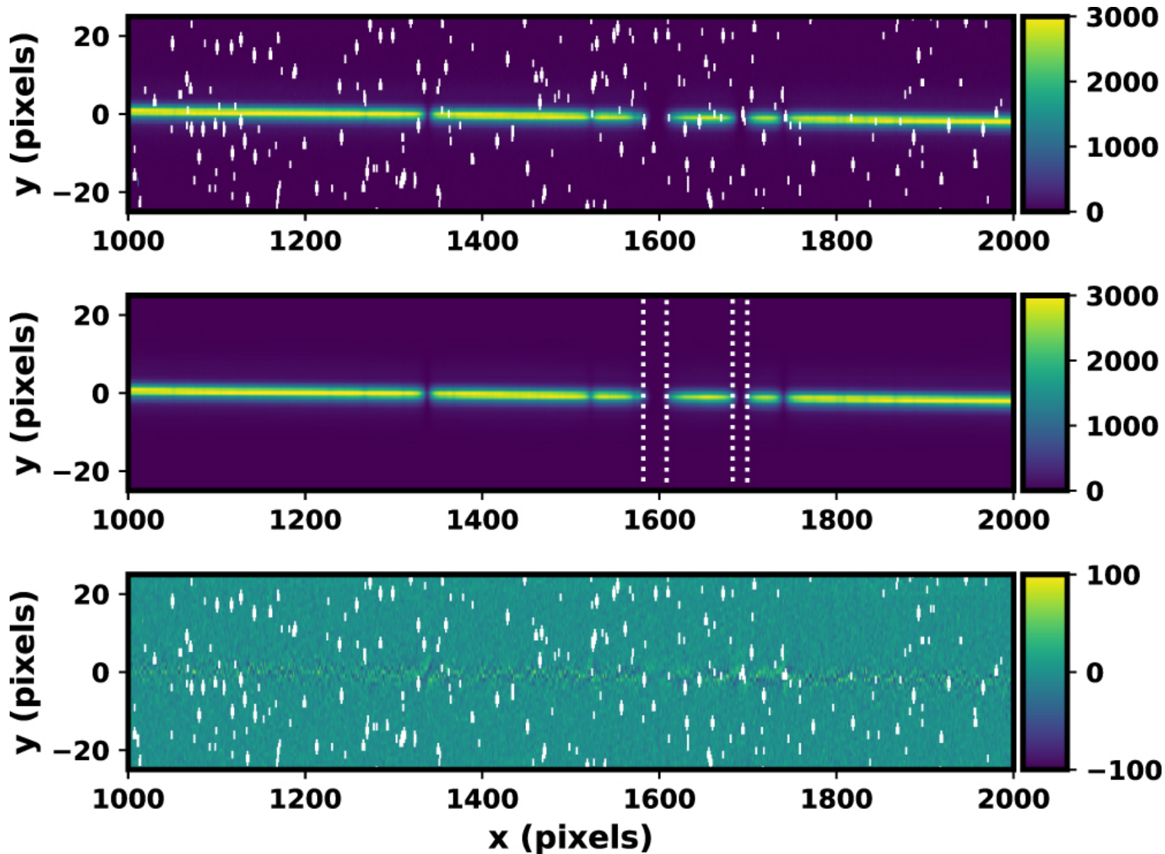
Figure 4. from Måns Holmberg and Nikku Madhusudhan 2022 Astron. J. 164 doi:10.3847/1538-3881/ac77eb https://dx.doi.org/10.3847/1538-3881/ac77eb © 2022. The Author(s). Published by the American Astronomical Society.
