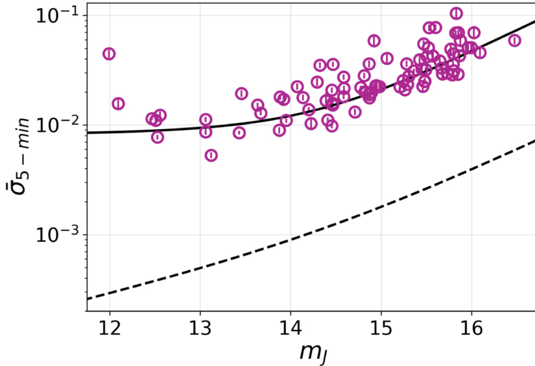
Figure 9. from Patrick Tamburo et al 2022 Astron. J. 163 doi:10.3847/1538-3881/ac64aa https://dx.doi.org/10.3847/1538-3881/ac64aa © 2022. The Author(s). Published by the American Astronomical Society.
