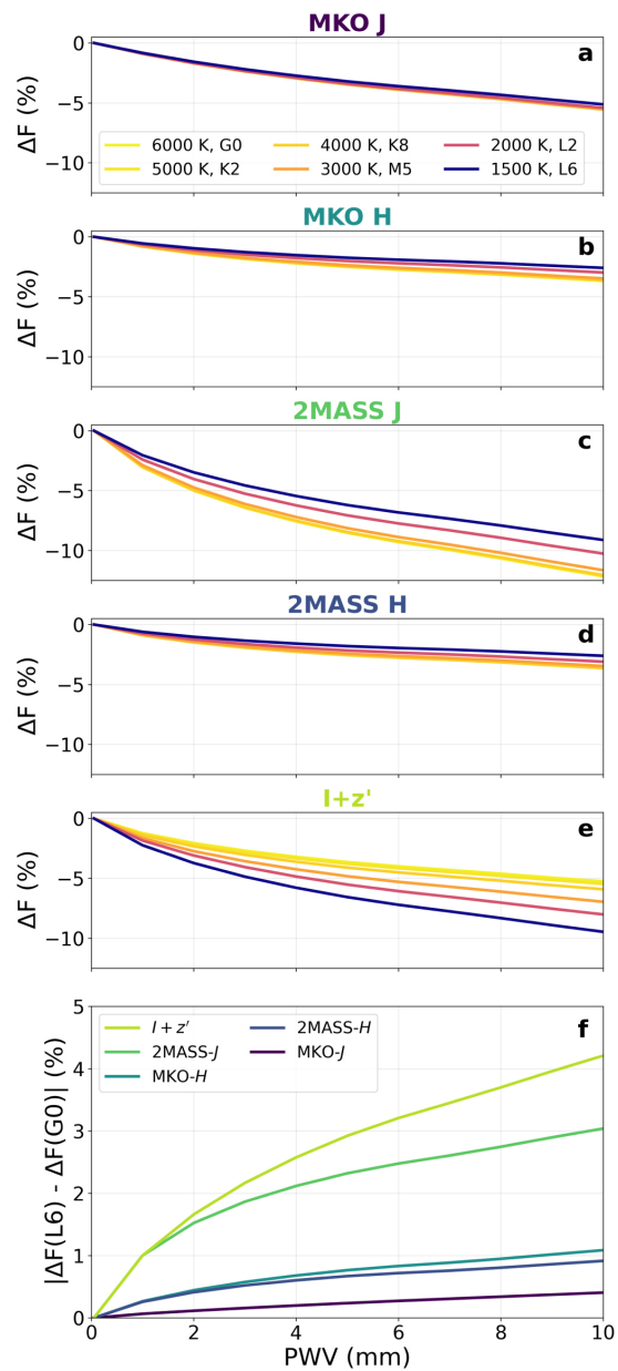
Figure 8. from Patrick Tamburo et al 2022 Astron. J. 163 doi:10.3847/1538-3881/ac64aa https://dx.doi.org/10.3847/1538-3881/ac64aa © 2022. The Author(s). Published by the American Astronomical Society.
