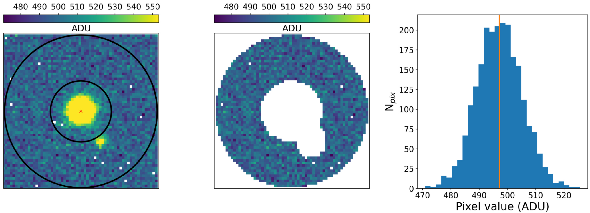
Figure 7. from Patrick Tamburo et al 2022 Astron. J. 163 doi:10.3847/1538-3881/ac64aa https://dx.doi.org/10.3847/1538-3881/ac64aa © 2022. The Author(s). Published by the American Astronomical Society.
