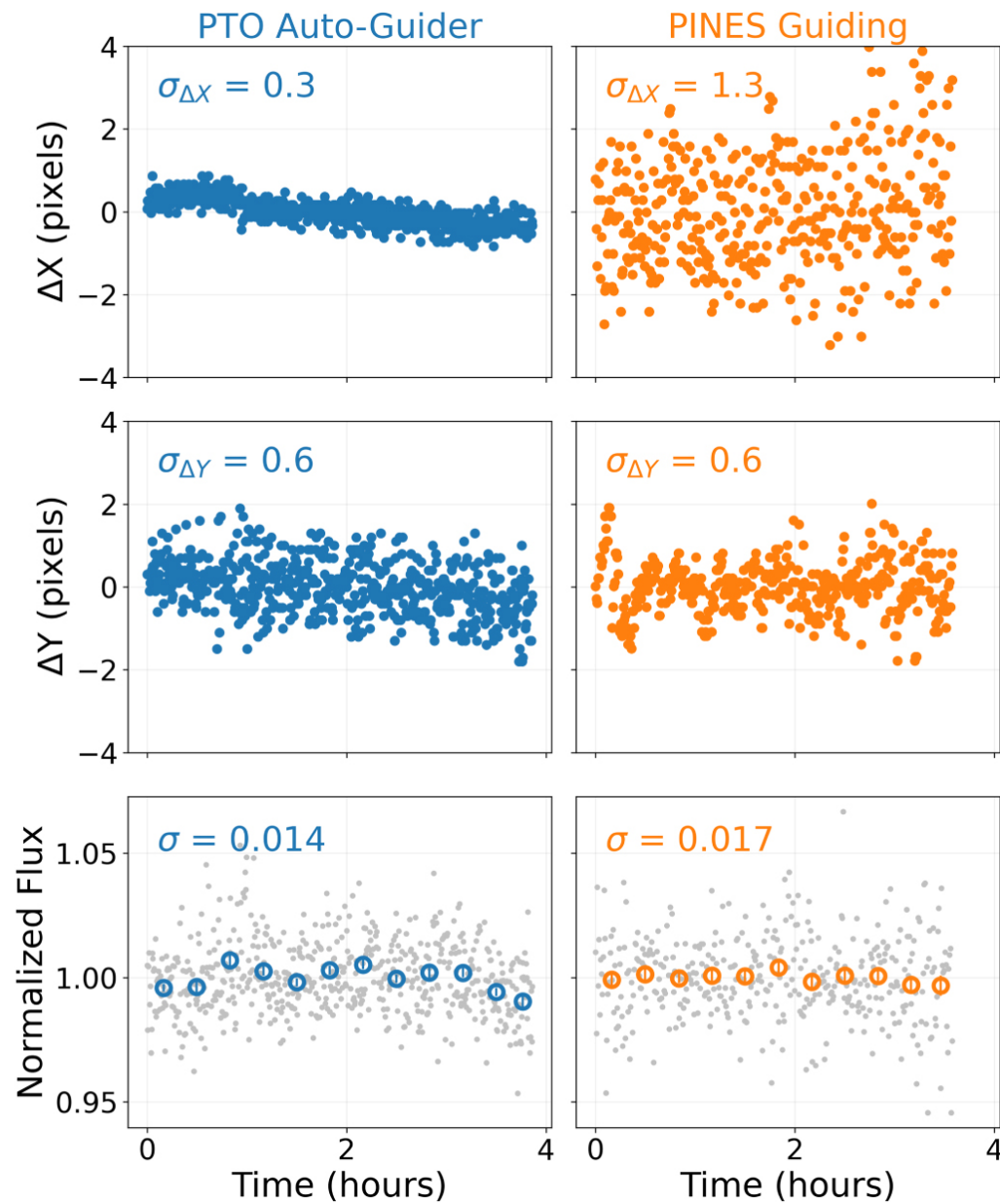
Figure 6. from Patrick Tamburo et al 2022 Astron. J. 163 doi:10.3847/1538-3881/ac64aa https://dx.doi.org/10.3847/1538-3881/ac64aa © 2022. The Author(s). Published by the American Astronomical Society.
