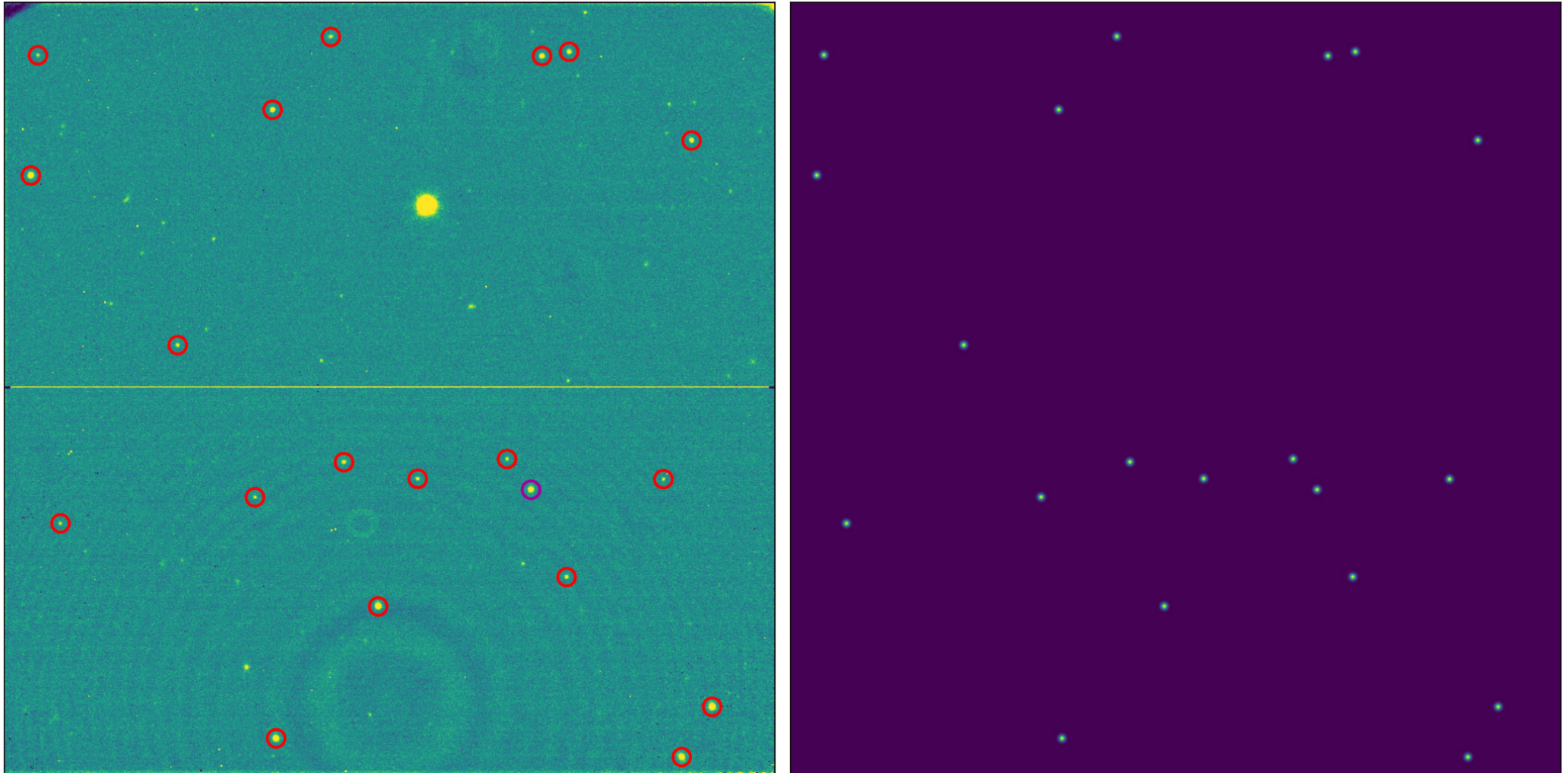
Figure 4. from Patrick Tamburo et al 2022 Astron. J. 163 doi:10.3847/1538-3881/ac64aa https://dx.doi.org/10.3847/1538-3881/ac64aa © 2022. The Author(s). Published by the American Astronomical Society.
