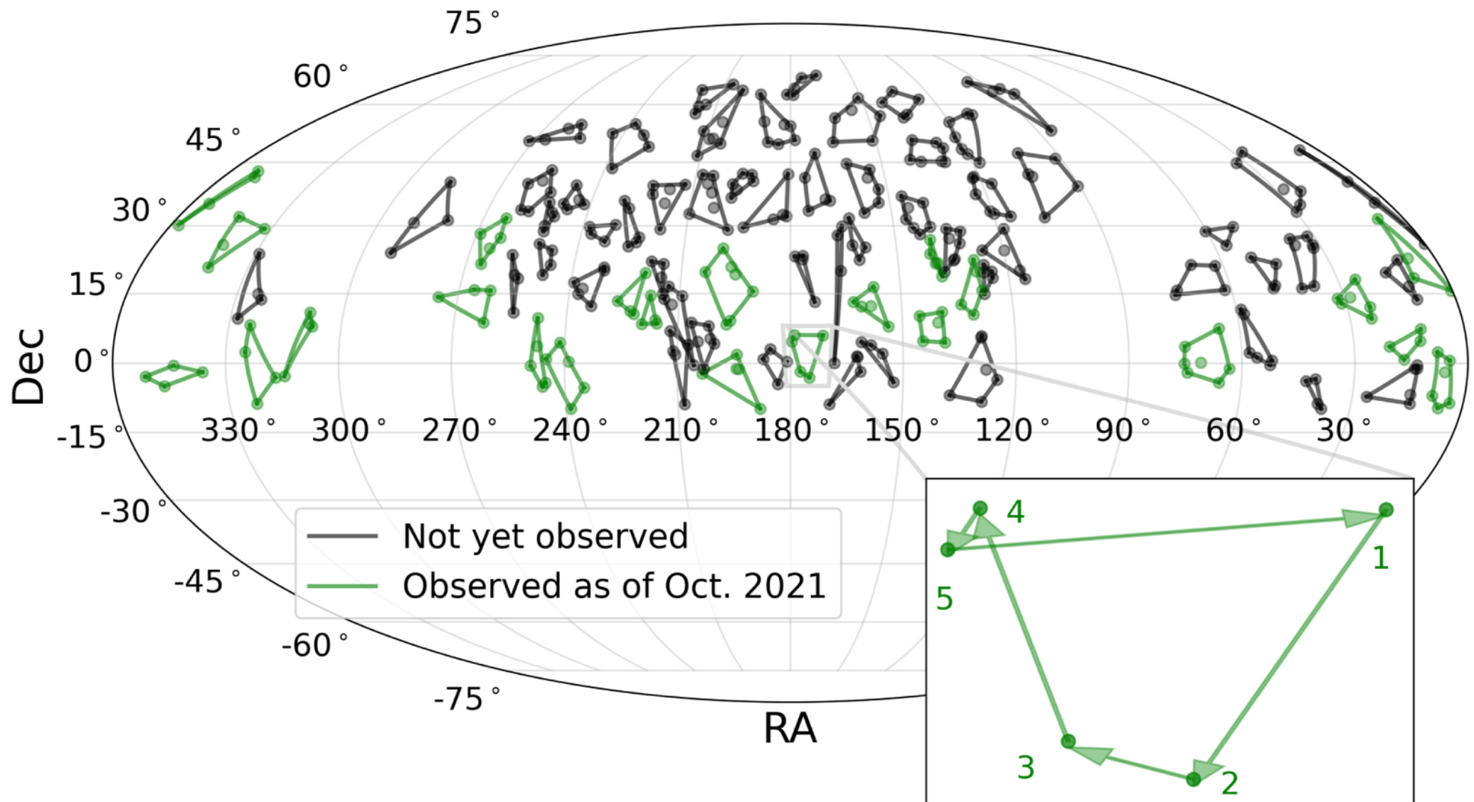
Figure 3. from Patrick Tamburo et al 2022 Astron. J. 163 doi:10.3847/1538-3881/ac64aa https://dx.doi.org/10.3847/1538-3881/ac64aa © 2022. The Author(s). Published by the American Astronomical Society.
