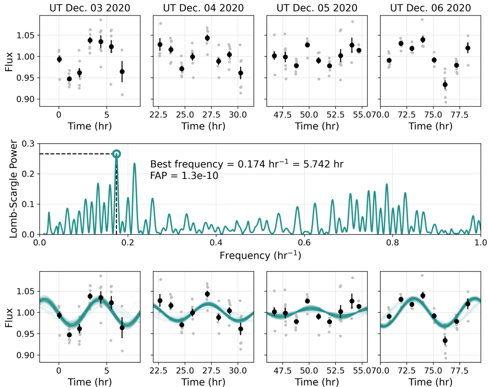
Figure 15. from Patrick Tamburo et al 2022 Astron. J. 163 doi:10.3847/1538-3881/ac64aa https://dx.doi.org/10.3847/1538-3881/ac64aa © 2022. The Author(s). Published by the American Astronomical Society.
