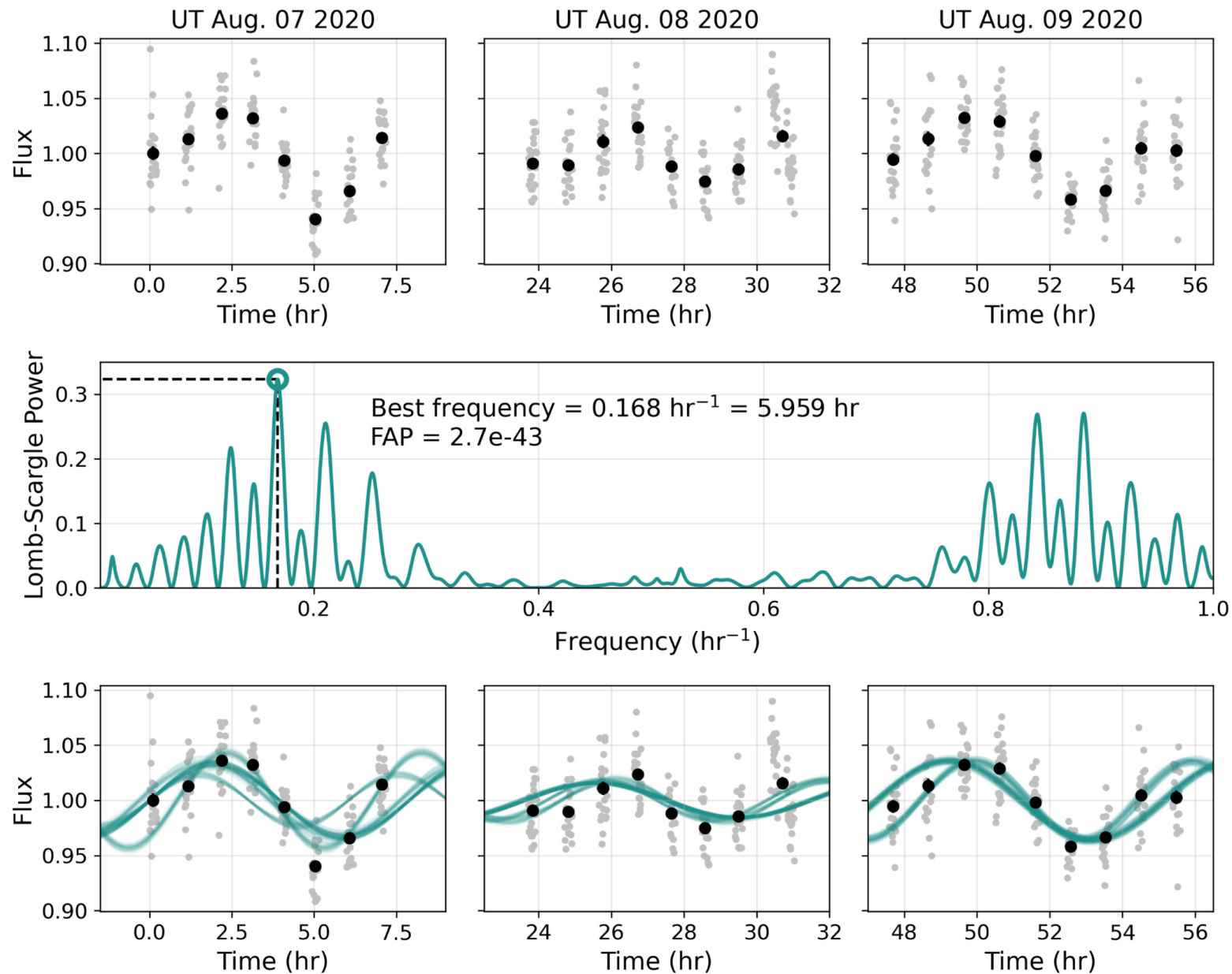
Figure 14. from Patrick Tamburo et al 2022 Astron. J. 163 doi:10.3847/1538-3881/ac64aa https://dx.doi.org/10.3847/1538-3881/ac64aa © 2022. The Author(s). Published by the American Astronomical Society.
