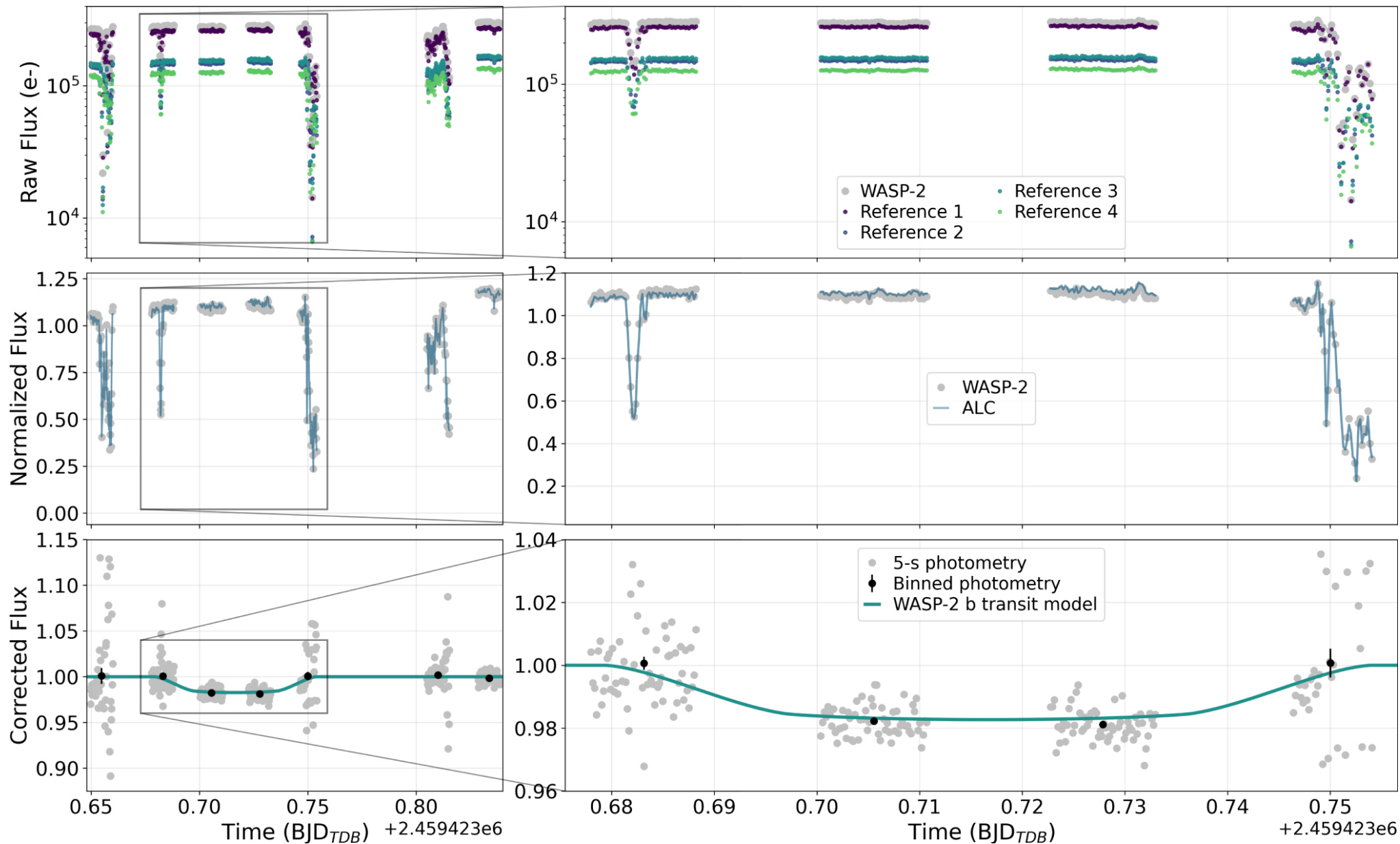
Figure 11. from Patrick Tamburo et al 2022 Astron. J. 163 doi:10.3847/1538-3881/ac64aa https://dx.doi.org/10.3847/1538-3881/ac64aa © 2022. The Author(s). Published by the American Astronomical Society.
