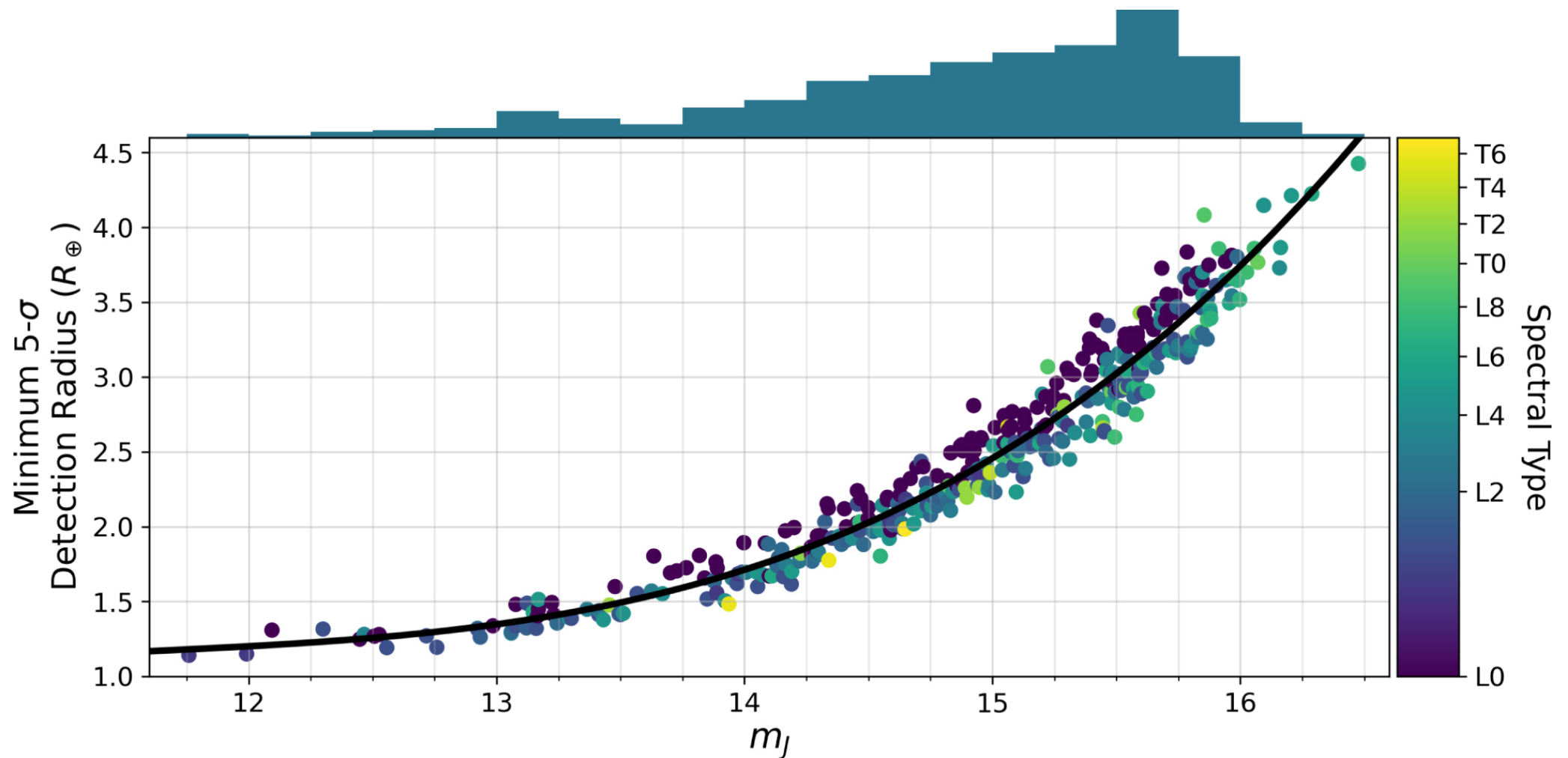
Figure 10. from Patrick Tamburo et al 2022 Astron. J. 163 doi:10.3847/1538-3881/ac64aa https://dx.doi.org/10.3847/1538-3881/ac64aa © 2022. The Author(s). Published by the American Astronomical Society.
