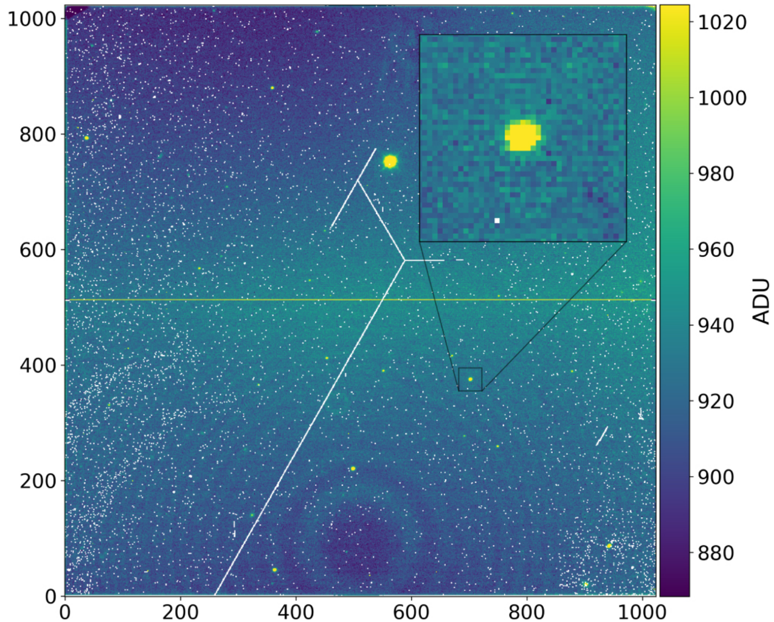
Figure 1. from Patrick Tamburo et al 2022 Astron. J. 163 doi:10.3847/1538-3881/ac64aa https://dx.doi.org/10.3847/1538-3881/ac64aa © 2022. The Author(s). Published by the American Astronomical Society.
